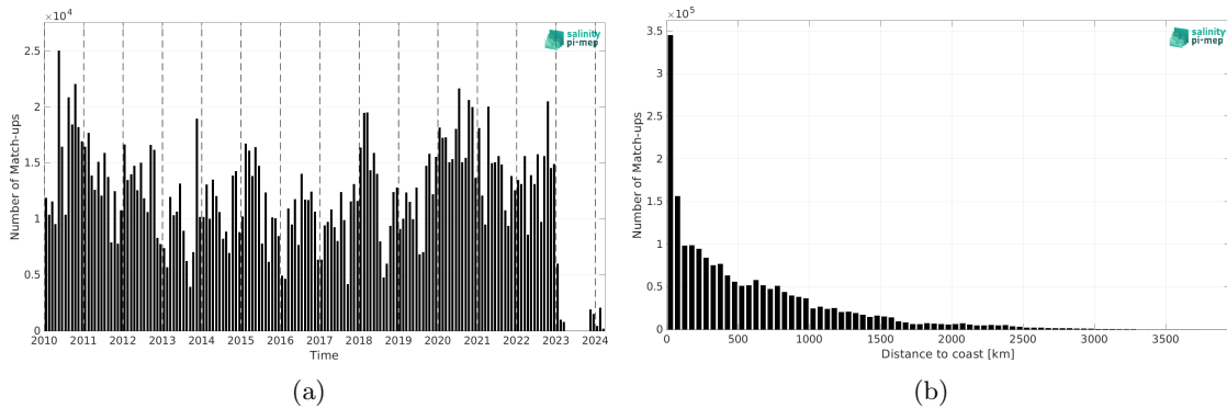
Figure 2: Number of match-ups between TSG (LEGOS-DM) and SMOS SSS L4 v1 - Daily (CMEMS-CNR) SSS as a function of time (a) and as function of the distance to coast (b) over the Pacific Ocean Pi-MEP region and for the full satellite product period.
