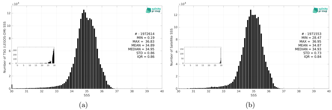
Figure 3: Histograms of SSS from TSG (LEGOS-DM) (a) and SMOS SSS L4 v1 - Daily (CMEMS-CNR) (b) considering all match-up pairs per bins of 0.1 over the Pacific Ocean Pi-MEP region and for the full satellite product period.
