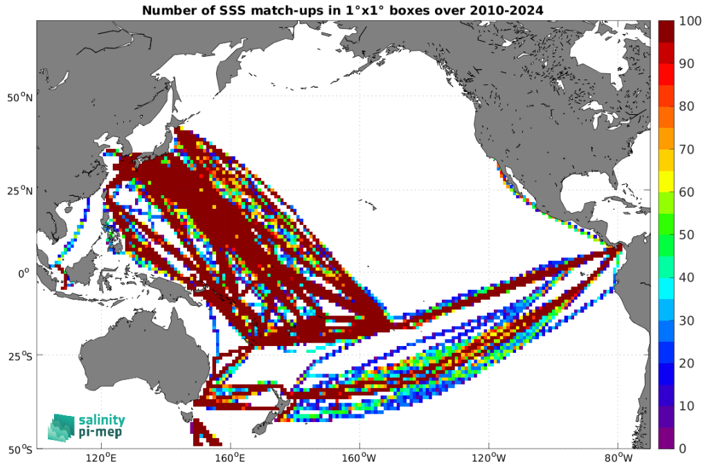
Figure 5: Number of SSS match-ups between TSG (LEGOS-DM) SSS and the SMOS SSS L4 v1 - Daily (CMEMS-CNR) SSS product for the Pacific Ocean Pi-MEP region over 1^\circ \times 1^\circ boxes and for the full satellite product period.
