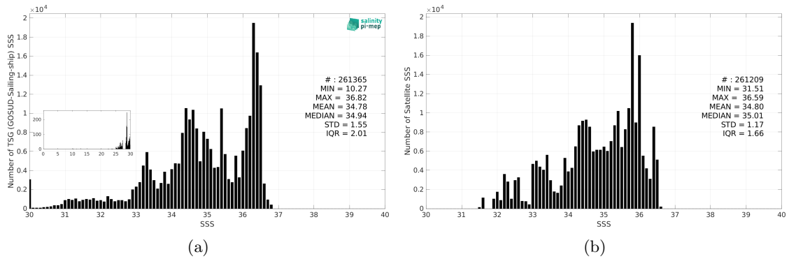
Figure 3: Histograms of SSS from TSG (GOSUD-Sailing-ship) (a) and SMOS SSS L4 v1 - Daily (CMEMS-CNR) (b) considering all match-up pairs per bins of 0.1 over the Pacific Ocean Pi-MEP region and for the full satellite product period.
