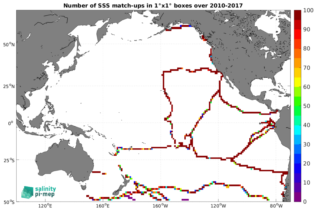
Figure 5: Number of SSS match-ups between TSG (GOSUD-Sailing-ship) SSS and the SMOS SSS L4 v1 - Daily (CMEMS-CNR) SSS product for the Pacific Ocean Pi-MEP region over 1^\circ \times 1^\circ boxes and for the full satellite product period.
