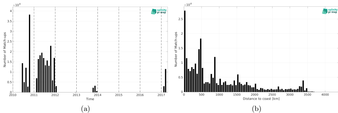
Figure 2: Number of match-ups between TSG (GOSUD-Sailing-ship) and SMOS SSS L4 v1 - Daily (CMEMS-CNR) SSS as a function of time (a) and as function of the distance to coast (b) over the Pacific Ocean Pi-MEP region and for the full satellite product period.
