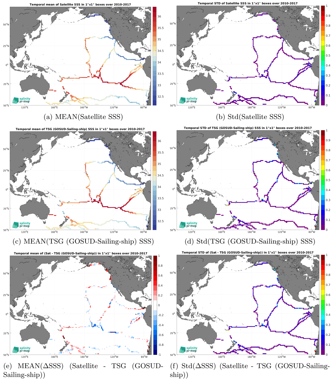
Figure 7: Temporal mean (left) and Std (right) of SSS from SMOS SSS L4 v1 - Daily (CMEMS-CNR) (top), TSG (GOSUD-Sailing-ship) (middle), and of \Delta SSS (Satellite - TSG (GOSUD-Sailing-ship)). Only match-up pairs are used to generate these maps.
