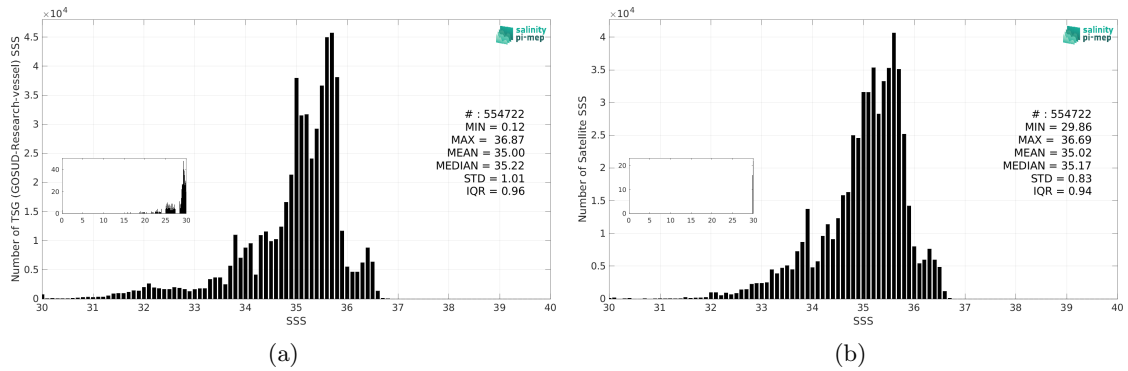
Figure 3: Histograms of SSS from TSG (GOSUD-Research-vessel) (a) and SMOS SSS L4 v1 - Daily (CMEMS-CNR) (b) considering all match-up pairs per bins of 0.1 over the Pacific Ocean Pi-MEP region and for the full satellite product period.
