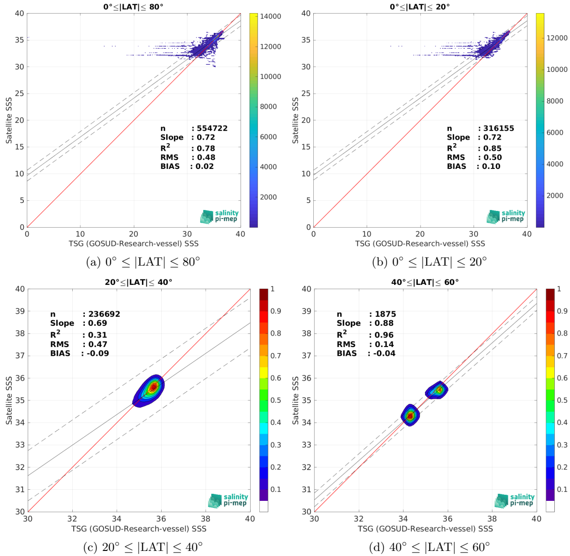
Figure 10: Contour maps of the concentration of SMOS SSS L4 v1 - Daily (CMEMS-CNR) SSS (y-axis) versus TSG (GOSUD-Research-vessel) SSS (x-axis) at match-up pairs for different latitude bands. For each plot, the red line shows x=y . The black thin and dashed lines indicate a linear fit through the data cloud and the \pm 95\% confidence levels, respectively. The number of match-up pairs n , the slope and R^2 coefficient of the linear fit, the root mean square (RMS) and the mean bias between satellite and in situ data are indicated for each latitude band in each plot.
