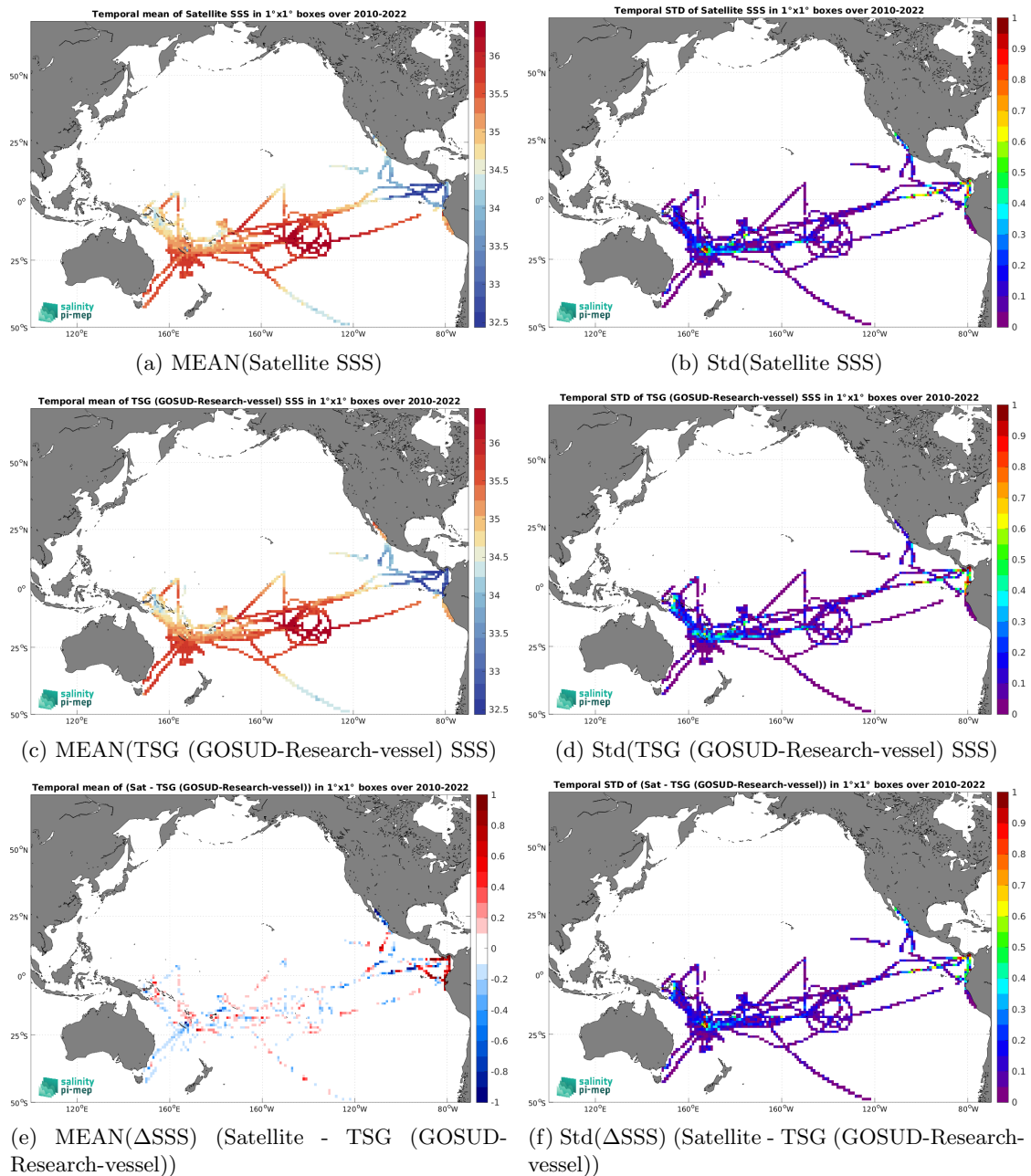
Figure 7: Temporal mean (left) and Std (right) of SSS from SMOS SSS L4 v1 - Daily (CMEMS-CNR) (top), TSG (GOSUD-Research-vessel) (middle), and of \Delta SSS (Satellite - TSG (GOSUD-Research-vessel)). Only match-up pairs are used to generate these maps.
