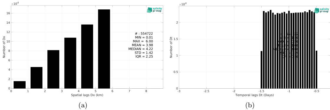
Figure 6: Histograms of the spatial (a) and temporal (b) lags between the location/time of the TSG (GOSUD-Research-vessel) measurement and the date of the corresponding SMOS SSS L4 v1 - Daily (CMEMS-CNR) SSS pixel.
