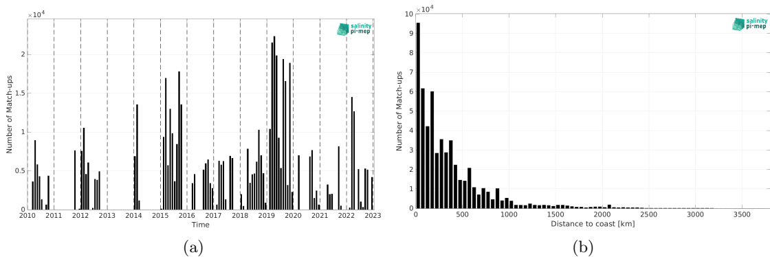
Figure 2: Number of match-ups between TSG (GOSUD-Research-vessel) and SMOS SSS L4 v1 - Daily (CMEMS-CNR) SSS as a function of time (a) and as function of the distance to coast (b) over the Pacific Ocean Pi-MEP region and for the full satellite product period.
