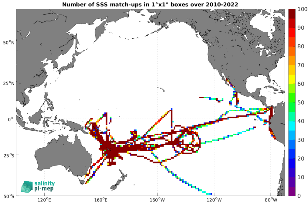
Figure 5: Number of SSS match-ups between TSG (GOSUD-Research-vessel) SSS and the SMOS SSS L4 v1 - Daily (CMEMS-CNR) SSS product for the Pacific Ocean Pi-MEP region over 1^\circ \times 1^\circ boxes and for the full satellite product period.
