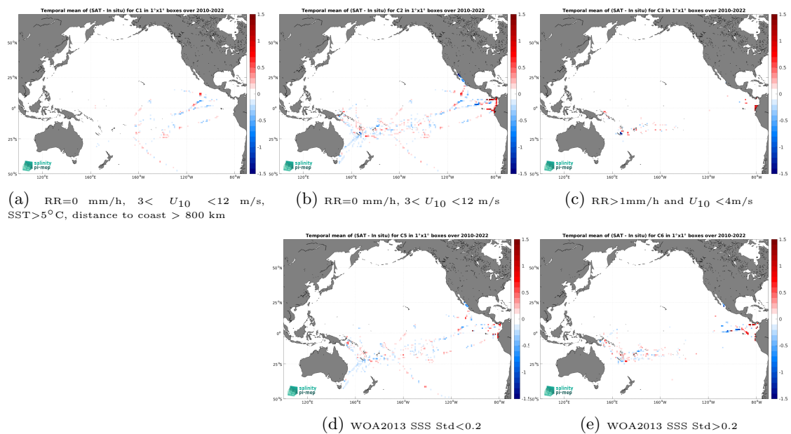
Figure 14: Temporal mean gridded over spatial boxes of size 1^\circ \times 1^\circ of \Delta SSS (SMOS SSS L4 v1 - Daily (CMEMS-CNR) - TSG (GOSUD-Research-vessel)) for 5 different subdatasets corresponding to:RR=0 mm/h, 3 < U_{10} < 12 m/s, SST > 5^\circ\text{C} , distance to coast > 800 km (a), RR=0 mm/h, 3 < U_{10} < 12 m/s (b), RR > 1 mm/h and U_{10} < 4 m/s (c), WOA2013 SSS Std < 0.2 (d), WOA2013 SSS Std > 0.2 (e).
