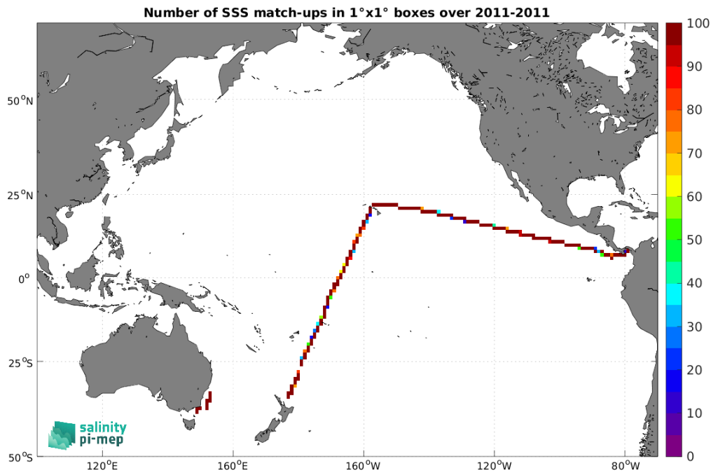
Figure 5: Number of SSS match-ups between TSG (CSIC-UTM) SSS and the SMOS SSS L4 v1 - Daily (CMEMS-CNR) SSS product for the Pacific Ocean Pi-MEP region over 1^\circ \times 1^\circ boxes and for the full satellite product period.
