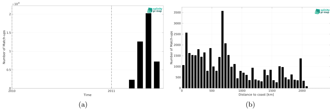
Figure 2: Number of match-ups between TSG (CSIC-UTM) and SMOS SSS L4 v1 - Daily (CMEMS-CNR) SSS as a function of time (a) and as function of the distance to coast (b) over the Pacific Ocean Pi-MEP region and for the full satellite product period.
