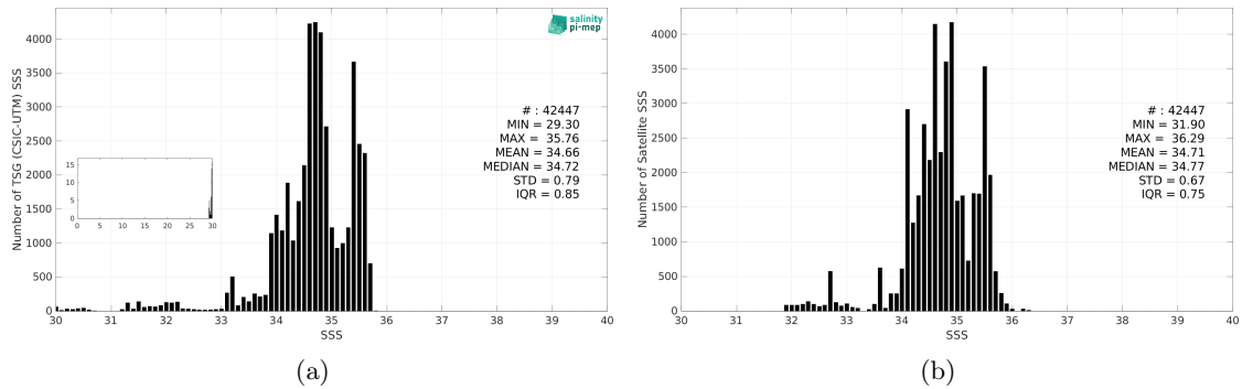
Figure 3: Histograms of SSS from TSG (CSIC-UTM) (a) and SMOS SSS L4 v1 - Daily (CMEMS-CNR) (b) considering all match-up pairs per bins of 0.1 over the Pacific Ocean Pi-MEP region and for the full satellite product period.
