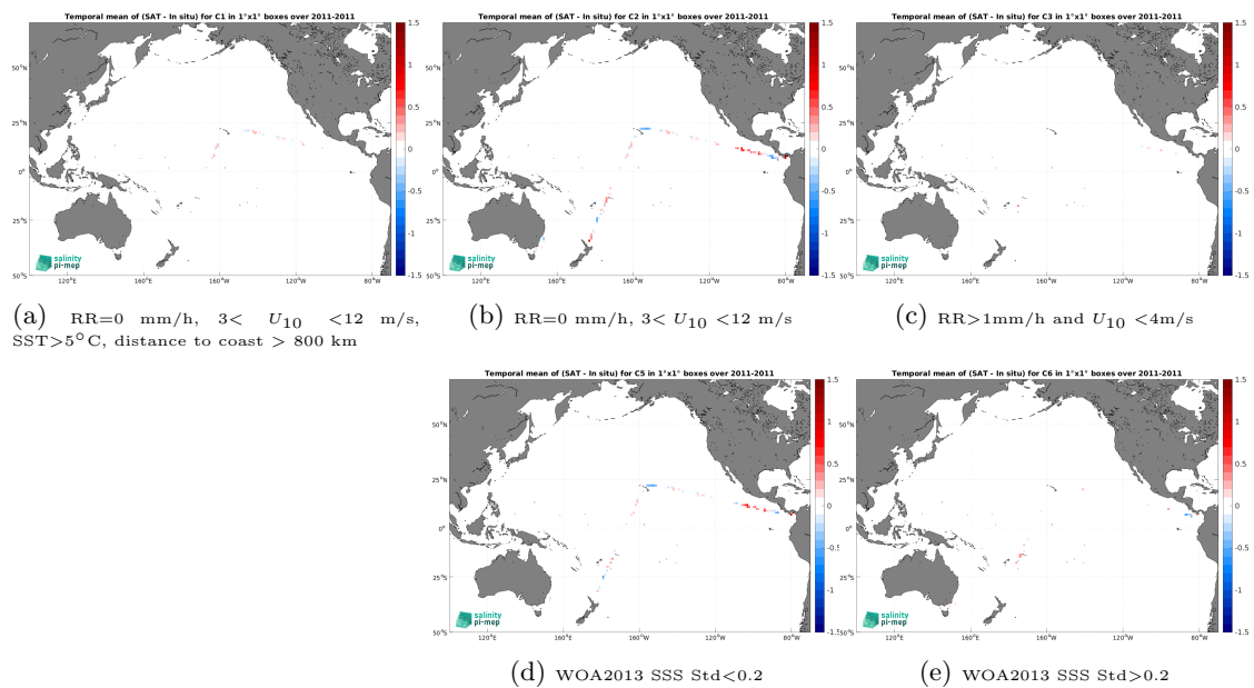
Figure 14: Temporal mean gridded over spatial boxes of size 1^\circ \times 1^\circ of \Delta SSS (SMOS SSS L4 v1 - Daily (CMEMS-CNR) - TSG (CSIC-UTM)) for 5 different subdatasets corresponding to: RR=0 mm/h, 3 < U_{10} < 12 m/s, SST > 5^\circ\text{C} , distance to coast > 800 km (a), RR=0 mm/h, 3 < U_{10} < 12 m/s (b), RR > 1 mm/h and U_{10} < 4 m/s (c), WOA2013 SSS Std < 0.2 (d), WOA2013 SSS Std > 0.2 (e).
