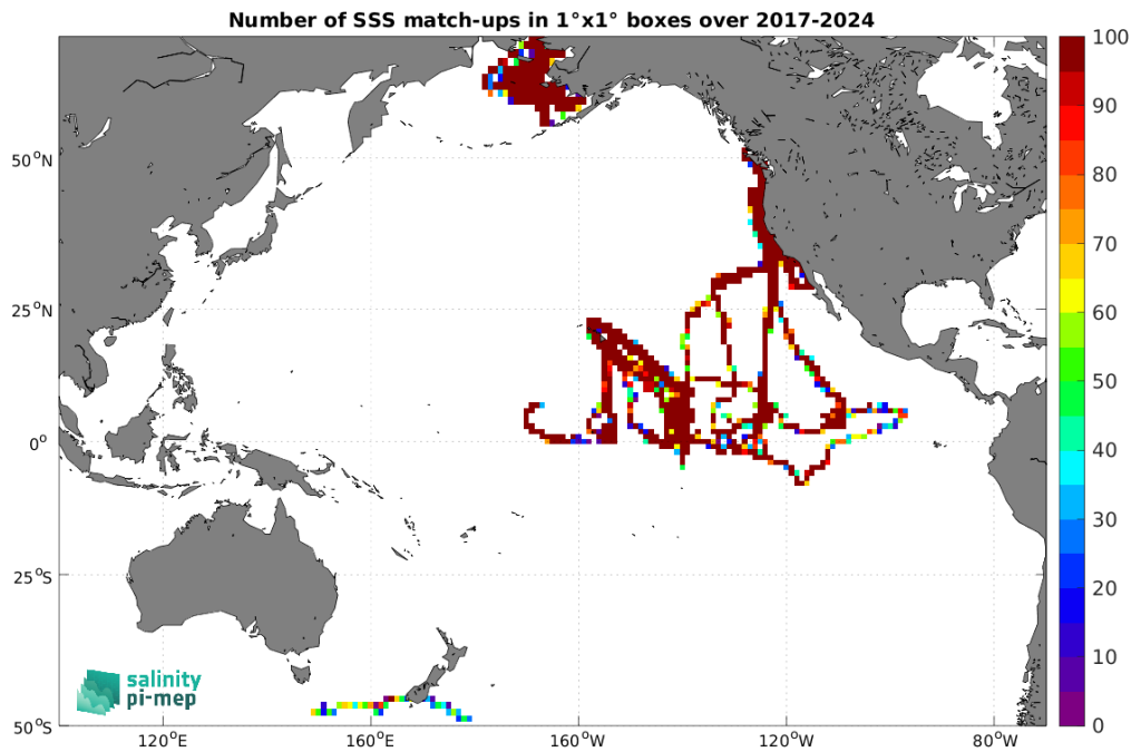
Figure 5: Number of SSS match-ups between Saildrone SSS and the SMOS SSS L4 v1 - Daily (CMEMS-CNR) SSS product for the Pacific Ocean Pi-MEP region over 1^\circ \times 1^\circ boxes and for the full satellite product period.
