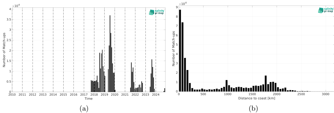
Figure 2: Number of match-ups between Saildrone and SMOS SSS L4 v1 - Daily (CMEMS-CNR) SSS as a function of time (a) and as function of the distance to coast (b) over the Pacific Ocean Pi-MEP region and for the full satellite product period.
