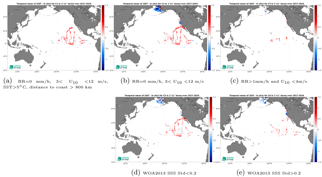
Figure 14: Temporal mean gridded over spatial boxes of size 1^\circ \times 1^\circ of \Delta SSS (SMOS SSS L4 v1 - Daily (CMEMS-CNR) - Saildrone) for 5 different subdatasets corresponding to:RR=0 mm/h, 3 < U_{10} < 12 m/s, SST >5^\circ\text{C} , distance to coast > 800 km (a), RR=0 mm/h, 3 < U_{10} < 12 m/s (b), RR >1 mm/h and U_{10} < 4 m/s (c), WOA2013 SSS Std <0.2 (d), WOA2013 SSS Std >0.2 (e).
