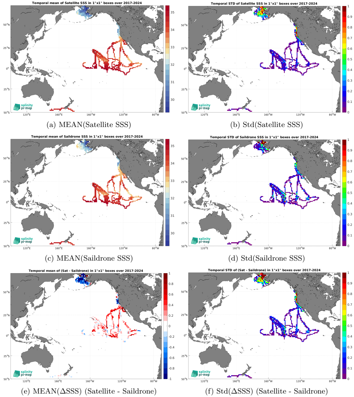
Figure 7: Temporal mean (left) and Std (right) of SSS from SMOS SSS L4 v1 - Daily (CMEMS-CNR) (top), Saildrone (middle), and of \Delta SSS (Satellite - Saildrone). Only match-up pairs are used to generate these maps.
