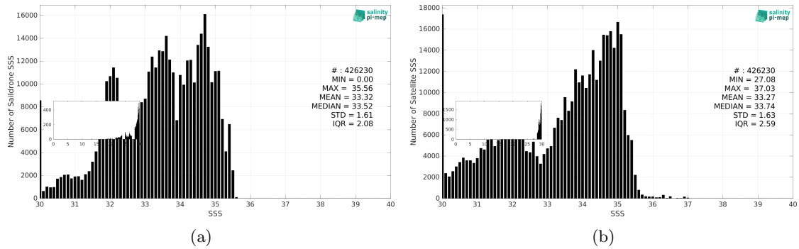
Figure 3: Histograms of SSS from Sairdrone (a) and SMOS SSS L4 v1 - Daily (CMEMS-CNR) (b) considering all match-up pairs per bins of 0.1 over the Pacific Ocean Pi-MEP region and for the full satellite product period.
