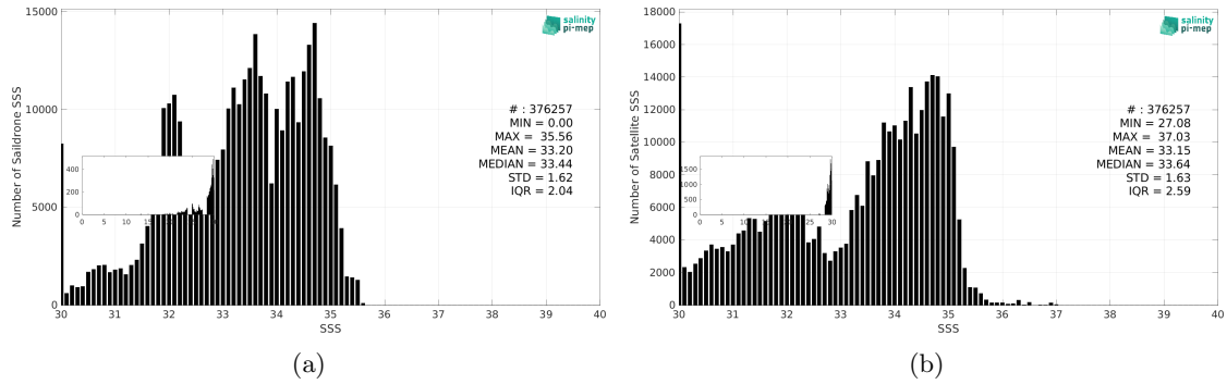
Figure 3: Histograms of SSS from Saildrone (a) and SMOS SSS L4 v1 - Daily (CMEMS-CNR) (b) considering all match-up pairs per bins of 0.1 over the Pacific Ocean Pi-MEP region and for the full satellite product period.
