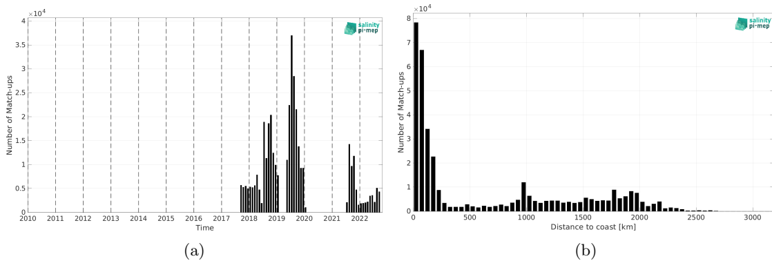
Figure 2: Number of match-ups between Sairdrone and SMOS SSS L4 v1 - Daily (CMEMS-CNR) SSS as a function of time (a) and as function of the distance to coast (b) over the Pacific Ocean Pi-MEP region and for the full satellite product period.
