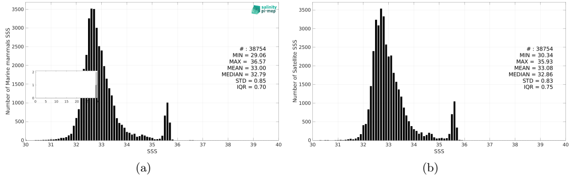
Figure 3: Histograms of SSS from Marine mammals (a) and SMOS SSS L4 v1 - Daily (CMEMS-CNR) (b) considering all match-up pairs per bins of 0.1 over the Pacific Ocean Pi-MEP region and for the full satellite product period.
