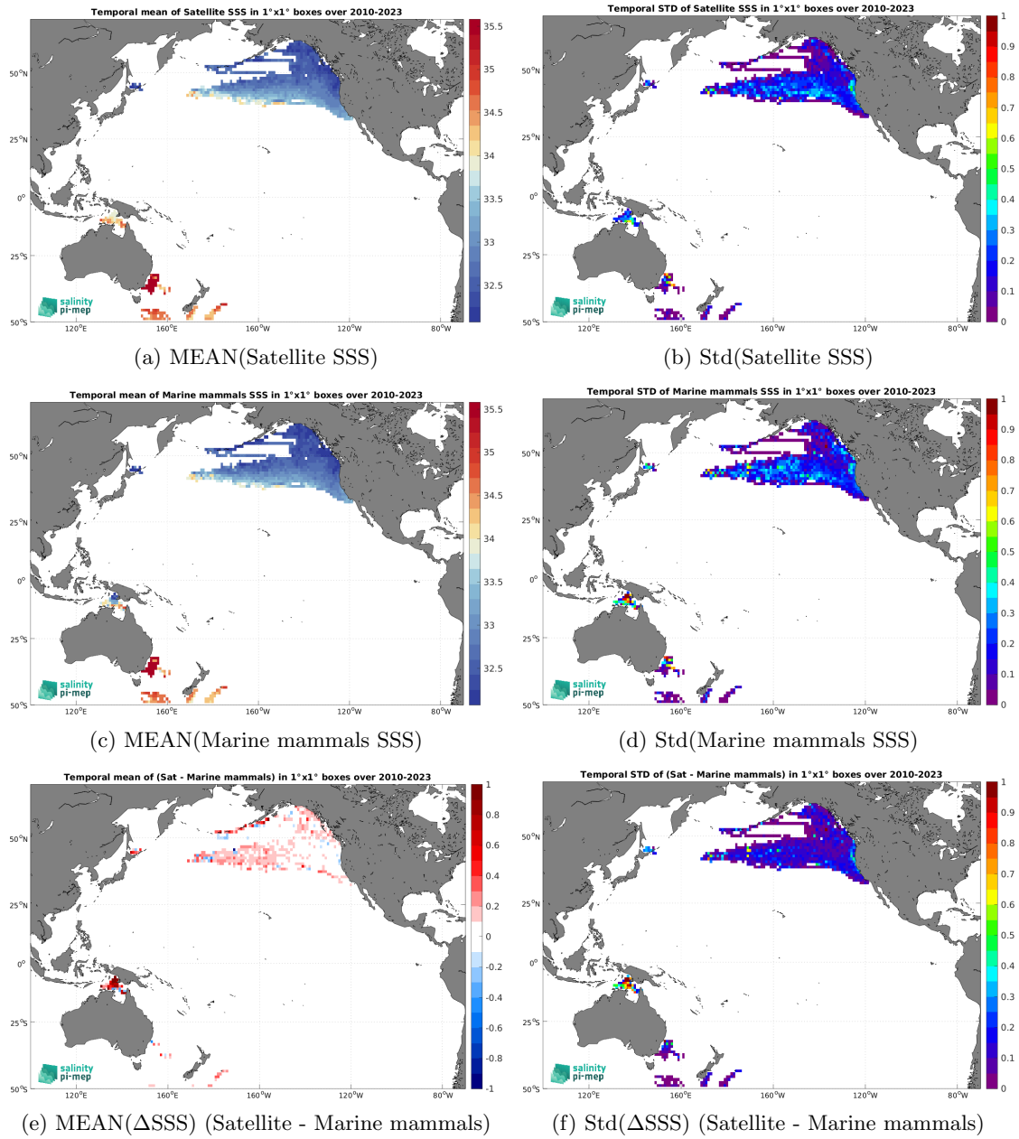
Figure 7: Temporal mean (left) and Std (right) of SSS from SMOS SSS L4 v1 - Daily (CMEMS-CNR) (top), Marine mammals (middle), and of \Delta SSS (Satellite - Marine mammals). Only match-up pairs are used to generate these maps.
