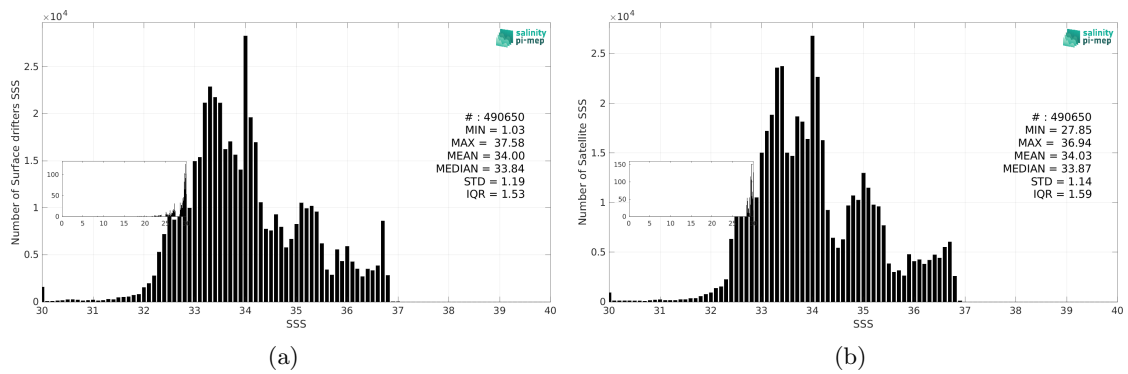
Figure 3: Histograms of SSS from Surface drifters (a) and SMOS SSS L4 v1 - Daily (CMEMS-CNR) (b) considering all match-up pairs per bins of 0.1 over the Pacific Ocean Pi-MEP region and for the full satellite product period.
