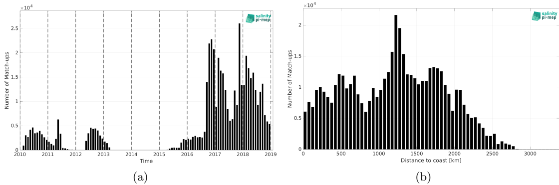
Figure 2: Number of match-ups between Surface drifters and SMOS SSS L4 v1 - Daily (CMEMS-CNR) SSS as a function of time (a) and as function of the distance to coast (b) over the Pacific Ocean Pi-MEP region and for the full satellite product period.
