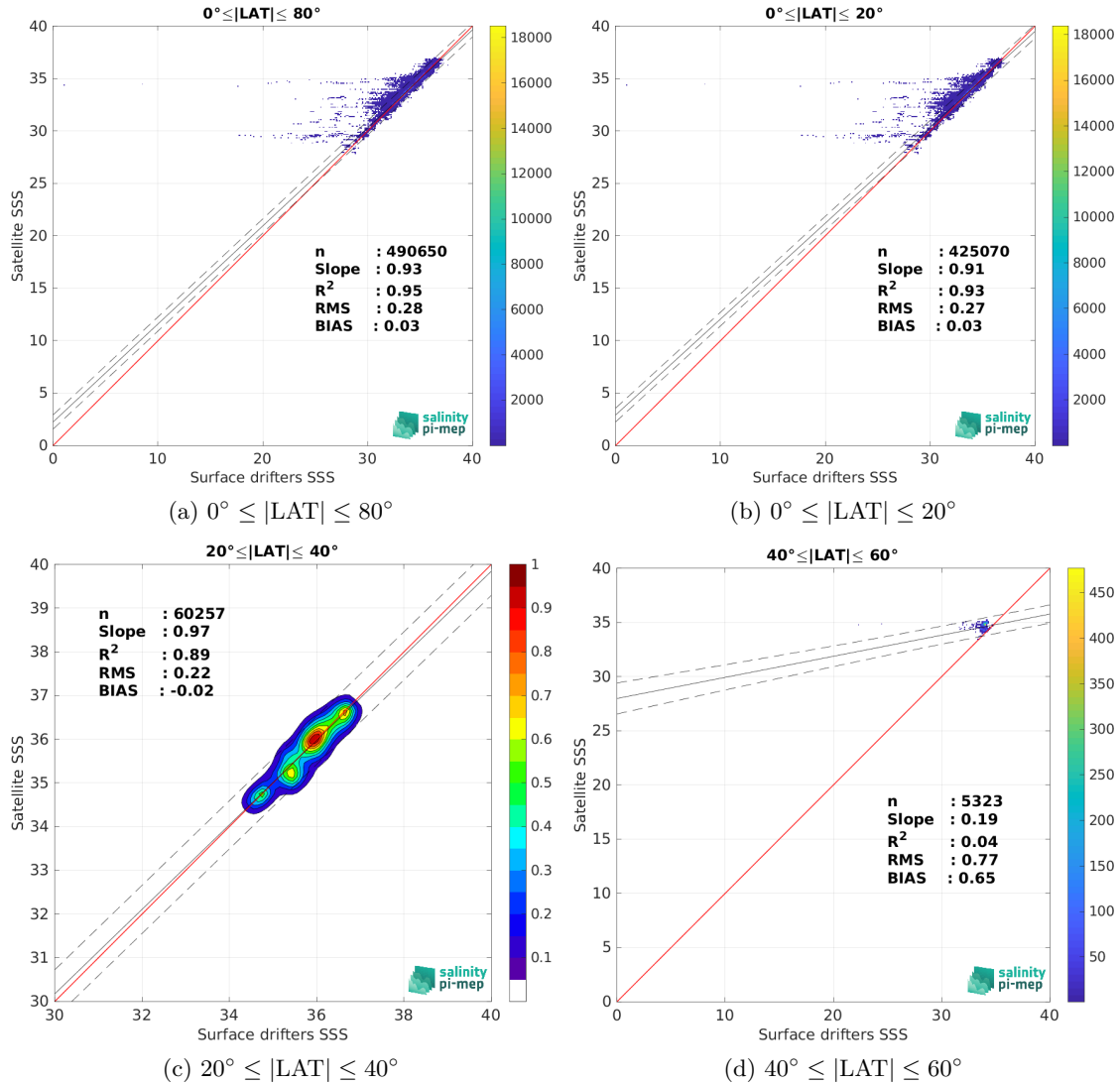
Figure 9: Contour maps of the concentration of SMOS SSS L4 v1 - Daily (CMEMS-CNR) SSS (y-axis) versus Surface drifters SSS (x-axis) at match-up pairs for different latitude bands. For each plot, the red line shows x=y . The black thin and dashed lines indicate a linear fit through the data cloud and the \pm 95\% confidence levels, respectively. The number match-up pairs n , the slope and R^2 coefficient of the linear fit, the root mean square (RMS) and the mean bias between satellite and in situ data are indicated for each latitude band in each plots.
