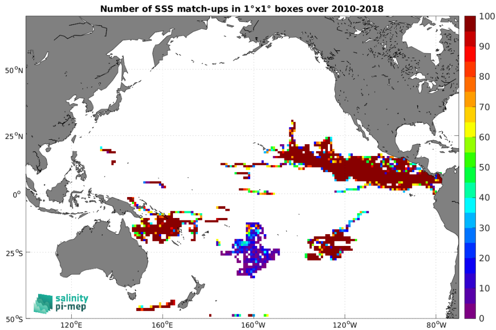
Figure 4: Number of SSS match-ups between Surface drifters SSS and the SMOS SSS L4 v1 - Daily (CMEMS-CNR) SSS product for the Pacific Ocean Pi-MEP region over 1^\circ \times 1^\circ boxes and for the full satellite product period.
