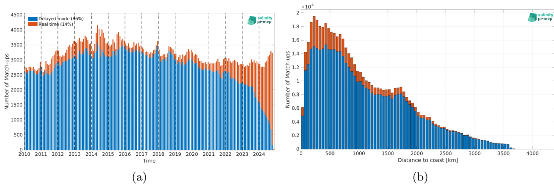
Figure 2: Number of match-ups between Argo and SMOS SSS L4 v1 - Daily (CMEMS-CNR) SSS as a function of time (a) and as function of the distance to coast (b) over the Pacific Ocean Pi-MEP region and for the full satellite product period.
