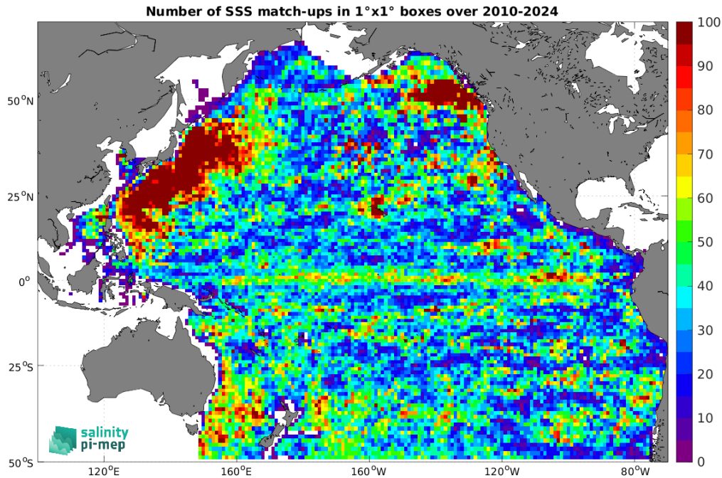
Figure 5: Number of SSS match-ups between Argo SSS and the SMOS SSS L4 v1 - Daily (CMEMS-CNR) SSS product for the Pacific Ocean Pi-MEP region over 1^\circ \times 1^\circ boxes and for the full satellite product period.
