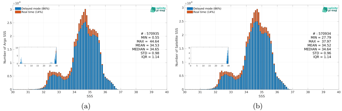
Figure 3: Histograms of SSS from Argo (a) and SMOS SSS L4 v1 - Daily (CMEMS-CNR) (b) considering all match-up pairs per bins of 0.1 over the Pacific Ocean Pi-MEP region and for the full satellite product period.
