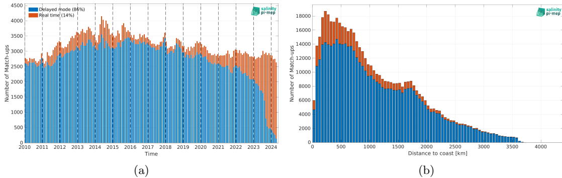
Figure 2: Number of match-ups between Argo and SMOS SSS L4 v1 - Daily (CMEMS-CNR) SSS as a function of time (a) and as function of the distance to coast (b) over the Pacific Ocean Pi-MEP region and for the full satellite product period.
