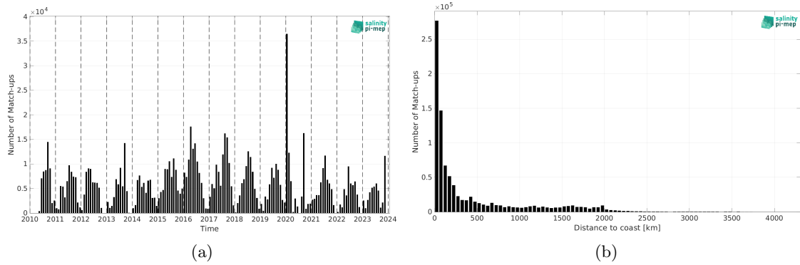
Figure 2: Number of match-ups between TSG (SAMOS) and SMOS SSS L4 OI v346 - Weekly (CMEMS-CATDS-LOPS) SSS as a function of time (a) and as function of the distance to coast (b) over the Pacific Ocean Pi-MEP region and for the full satellite product period.
