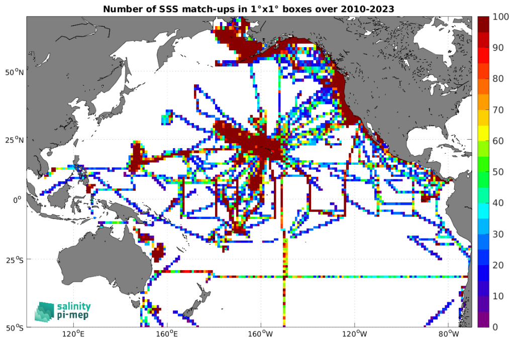
Figure 5: Number of SSS match-ups between TSG (SAMOS) SSS and the SMOS SSS L4 OI v346 - Weekly (CMEMS-CATDS-LOPS) SSS product for the Pacific Ocean Pi-MEP region over 1^\circ \times 1^\circ boxes and for the full satellite product period.
