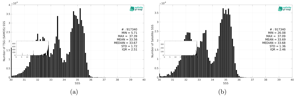
Figure 3: Histograms of SSS from TSG (SAMOS) (a) and SMOS SSS L4 OI v346 - Weekly (CMEMS-CATDS-LOPS) (b) considering all match-up pairs per bins of 0.1 over the Pacific Ocean Pi-MEP region and for the full satellite product period.
