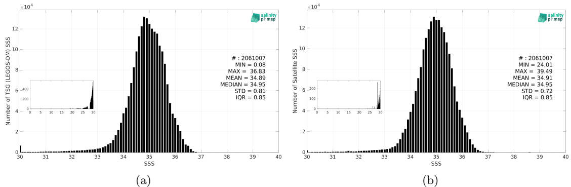
Figure 3: Histograms of SSS from TSG (LEGOS-DM) (a) and SMOS SSS L4 OI v346 - Weekly (CMEMS-CATDS-LOPS) (b) considering all match-up pairs per bins of 0.1 over the Pacific Ocean Pi-MEP region and for the full satellite product period.
