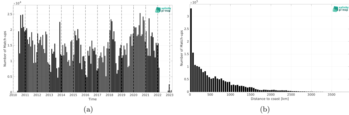
Figure 2: Number of match-ups between TSG (LEGOS-DM) and SMOS SSS L4 OI v346 - Weekly (CMEMS-CATDS-LOPS) SSS as a function of time (a) and as function of the distance to coast (b) over the Pacific Ocean Pi-MEP region and for the full satellite product period.
