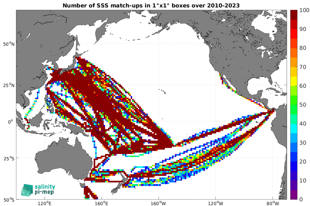
Figure 5: Number of SSS match-ups between TSG (LEGOS-DM) SSS and the SMOS SSS L4 OI v346 - Weekly (CMEMS-CATDS-LOPS) SSS product for the Pacific Ocean Pi-MEP region over 1^\circ \times 1^\circ boxes and for the full satellite product period.
