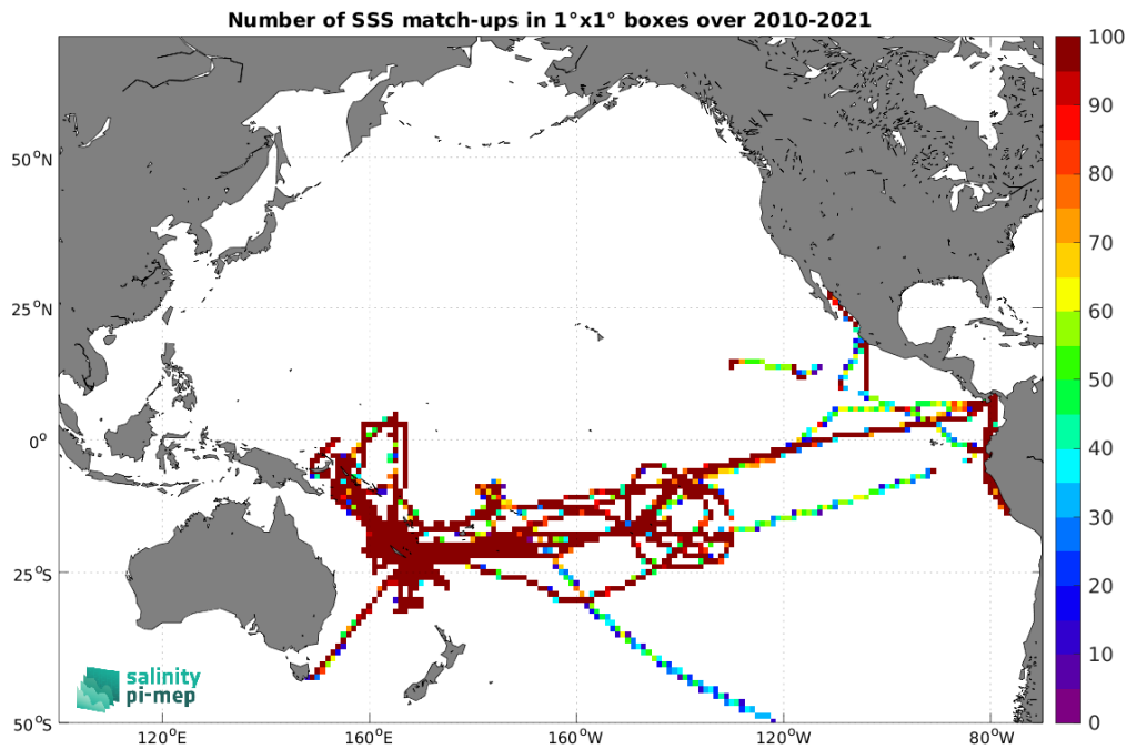
Figure 5: Number of SSS match-ups between TSG (GOSUD-Research-vessel) SSS and the SMOS SSS L4 OI v346 - Weekly (CMEMS-CATDS-LOPS) SSS product for the Pacific Ocean Pi-MEP region over 1^\circ \times 1^\circ boxes and for the full satellite product period.
