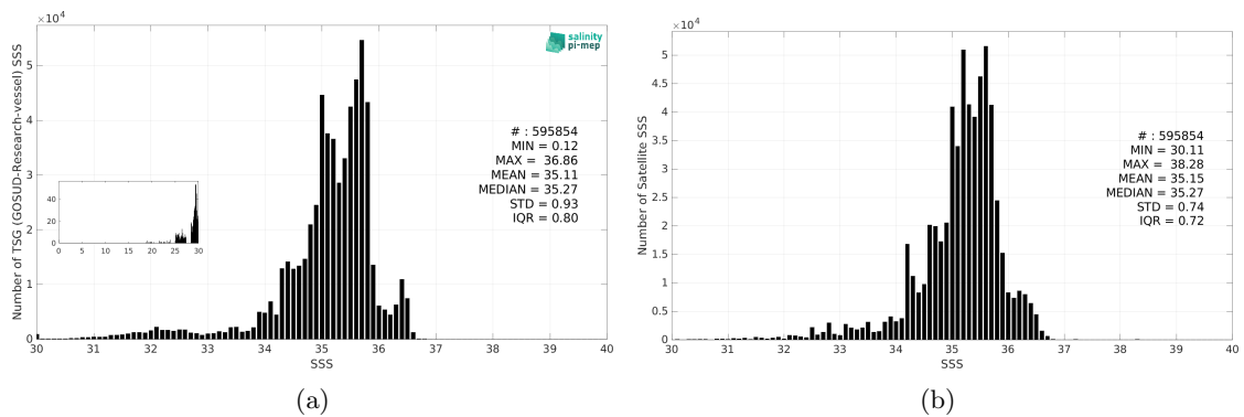
Figure 3: Histograms of SSS from TSG (GOSUD-Research-vessel) (a) and SMOS SSS L4 OI v346 - Weekly (CMEMS-CATDS-LOPS) (b) considering all match-up pairs per bins of 0.1 over the Pacific Ocean Pi-MEP region and for the full satellite product period.
