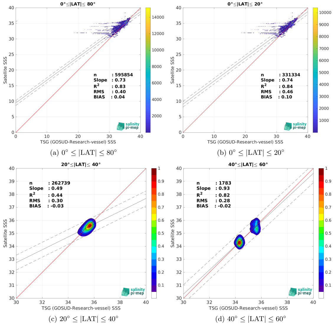
Figure 10: Contour maps of the concentration of SMOS SSS L4 OI v346 - Weekly (CMEMS-CATDS-LOPS) SSS (y-axis) versus TSG (GOSUD-Research-vessel) SSS (x-axis) at match-up pairs for different latitude bands. For each plot, the red line shows x=y . The black thin and dashed lines indicate a linear fit through the data cloud and the \pm 95\% confidence levels, respectively. The number match-up pairs n , the slope and R^2 coefficient of the linear fit, the root mean square (RMS) and the mean bias between satellite and in situ data are indicated for each latitude band in each plots.
