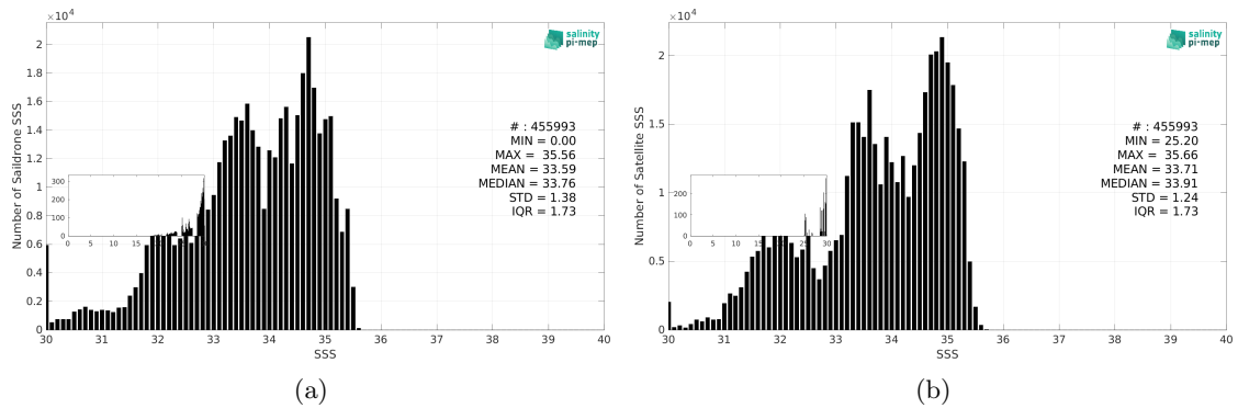
Figure 3: Histograms of SSS from Sailldrone (a) and SMOS SSS L4 OI v346 - Weekly (CMEMS-CATDS-LOPS) (b) considering all match-up pairs per bins of 0.1 over the Pacific Ocean Pi-MEP region and for the full satellite product period.
