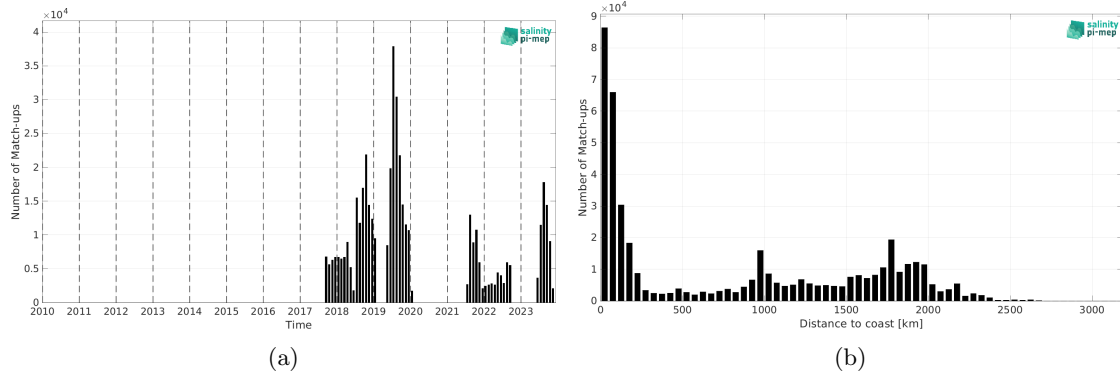
Figure 2: Number of match-ups between Sailldrone and SMOS SSS L4 OI v346 - Weekly (CMEMS-CATDS-LOPS) SSS as a function of time (a) and as function of the distance to coast (b) over the Pacific Ocean Pi-MEP region and for the full satellite product period.
