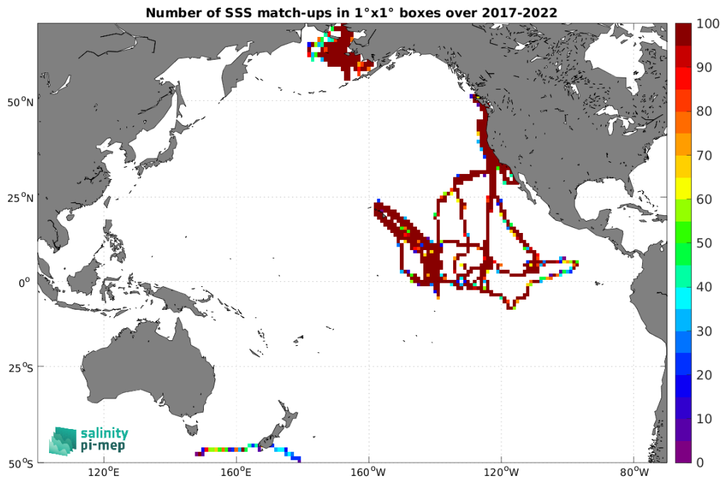
Figure 5: Number of SSS match-ups between Saildrone SSS and the SMOS SSS L4 OI v346 - Weekly (CMEMS-CATDS-LOPS) SSS product for the Pacific Ocean Pi-MEP region over 1^\circ \times 1^\circ boxes and for the full satellite product period.
