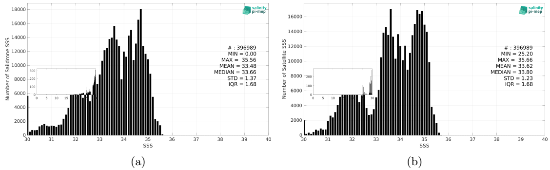
Figure 3: Histograms of SSS from Saildrone (a) and SMOS SSS L4 OI v346 - Weekly (CMEMS-CATDS-LOPS) (b) considering all match-up pairs per bins of 0.1 over the Pacific Ocean Pi-MEP region and for the full satellite product period.
