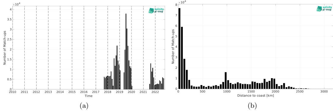
Figure 2: Number of match-ups between Saildrone and SMOS SSS L4 OI v346 - Weekly (CMEMS-CATDS-LOPS) SSS as a function of time (a) and as function of the distance to coast (b) over the Pacific Ocean Pi-MEP region and for the full satellite product period.
