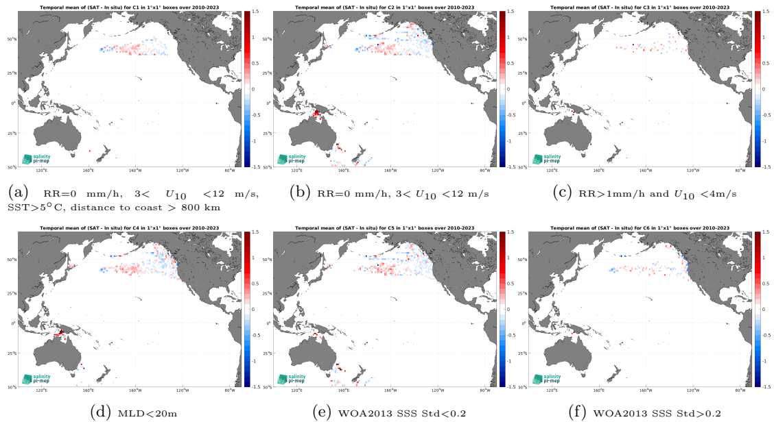
Figure 14: Temporal mean gridded over spatial boxes of size 1^\circ \times 1^\circ of \Delta\text{SSS} (SMOS SSS L4 OI v346 - Weekly (CMEMS-CATDS-LOPS) - Marine mammals) for 6 different subdatasets corresponding to:RR=0 mm/h, 3 < U_{10} < 12 m/s, SST>5°C, distance to coast > 800 km (a), RR=0 mm/h, 3 < U_{10} < 12 m/s (b), RR>1mm/h and U_{10} < 4 m/s (c),MLD<20m (d),WOA2013 SSS Std<0.2 (e),WOA2013 SSS Std>0.2 (f).
