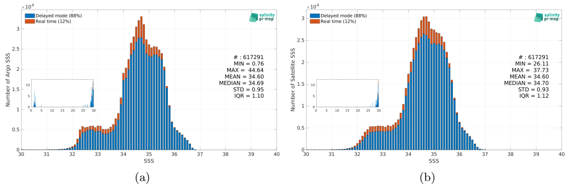
Figure 3: Histograms of SSS from Argo (a) and SMOS SSS L4 OI v346 - Weekly (CMEMS-CATDS-LOPS) (b) considering all match-up pairs per bins of 0.1 over the Pacific Ocean Pi-MEP region and for the full satellite product period.
