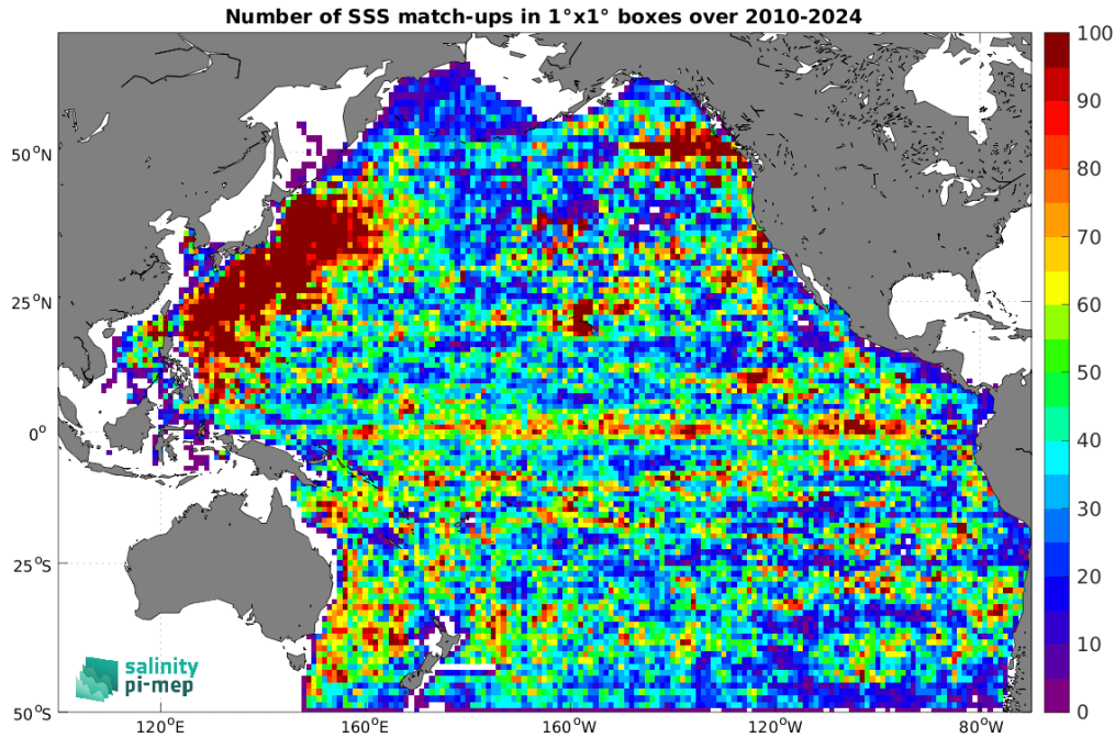
Figure 5: Number of SSS match-ups between Argo SSS and the SMOS SSS L4 OI v346 - Weekly (CMEMS-CATDS-LOPS) SSS product for the Pacific Ocean Pi-MEP region over 1^\circ \times 1^\circ boxes and for the full satellite product period.
