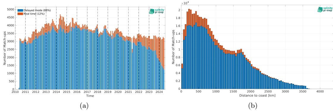
Figure 2: Number of match-ups between Argo and SMOS SSS L4 OI v346 - Weekly (CMEMS-CATDS-LOPS) SSS as a function of time (a) and as function of the distance to coast (b) over the Pacific Ocean Pi-MEP region and for the full satellite product period.
