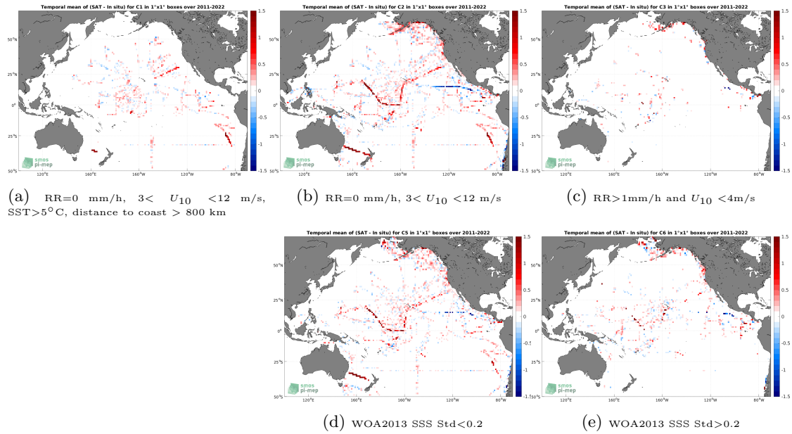
Figure 12: Temporal mean gridded over spatial boxes of size 1^\circ \times 1^\circ of \Delta\text{SSS} (SMOS SSS L4 OI v342 - Weekly (CMEMS-CATDS-LOPS) - TSG (SAMOS)) for 5 different subdatasets corresponding to:RR=0 mm/h, 3 < U_{10} < 12 m/s, SST >5^\circ\text{C} , distance to coast > 800 km (a), RR=0 mm/h, 3 < U_{10} < 12 m/s (b), RR >1 mm/h and U_{10} < 4 m/s (c), WOA2013 SSS Std <0.2 (d), WOA2013 SSS Std >0.2 (e).
