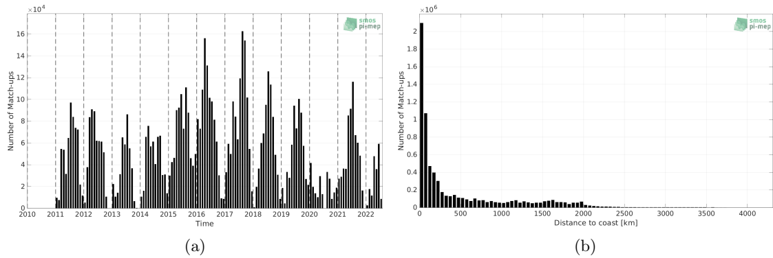
Figure 1: Number of match-ups between TSG (SAMOS) and SMOS SSS L4 OI v342 - Weekly (CMEMS-CATDS-LOPS) SSS as a function of time (a) and as function of the distance to coast (b) over the Pacific Ocean Pi-MEP region and for the full satellite product period.
