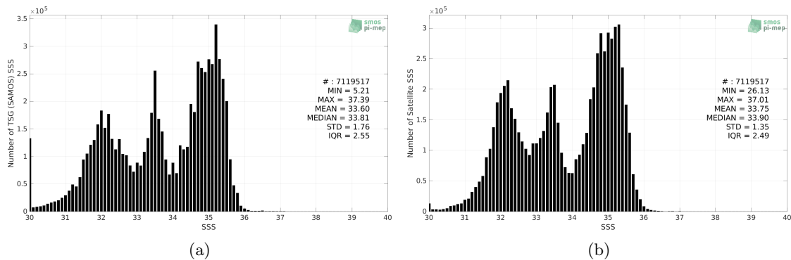
Figure 2: Histograms of SSS from TSG (SAMOS) (a) and SMOS SSS L4 OI v342 - Weekly (CMEMS-CATDS-LOPS) (b) considering all match-up pairs per bins of 0.1 over the Pacific Ocean Pi-MEP region and for the full satellite product period.
