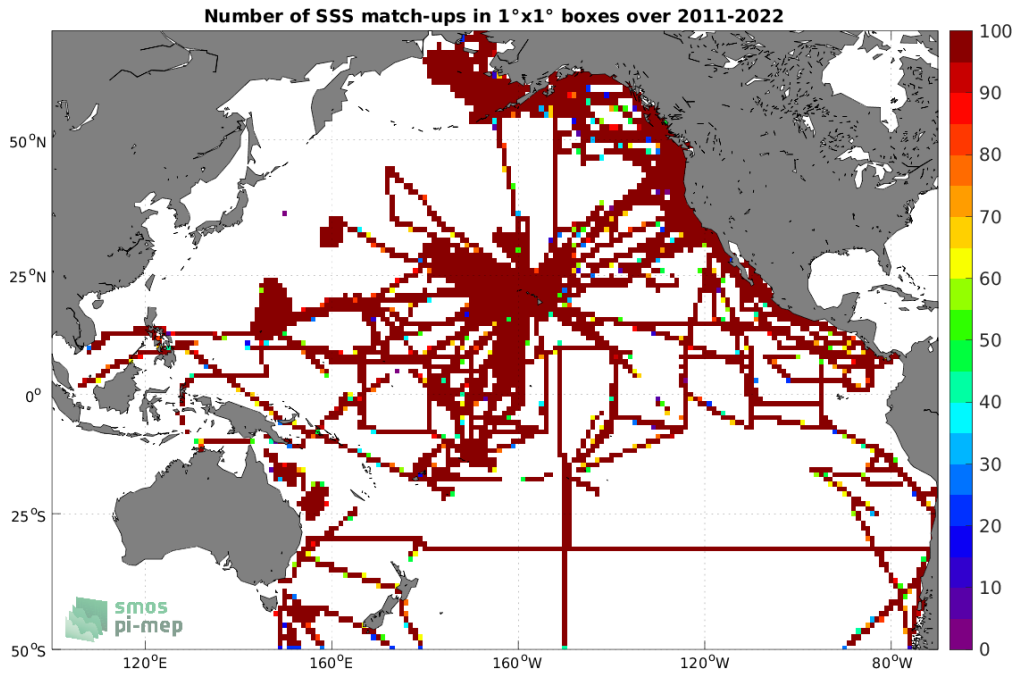
Figure 4: Number of SSS match-ups between TSG (SAMOS) SSS and the SMOS SSS L4 OI v342 - Weekly (CMEMS-CATDS-LOPS) SSS product for the Pacific Ocean Pi-MEP region over 1^\circ \times 1^\circ boxes and for the full satellite product period.
