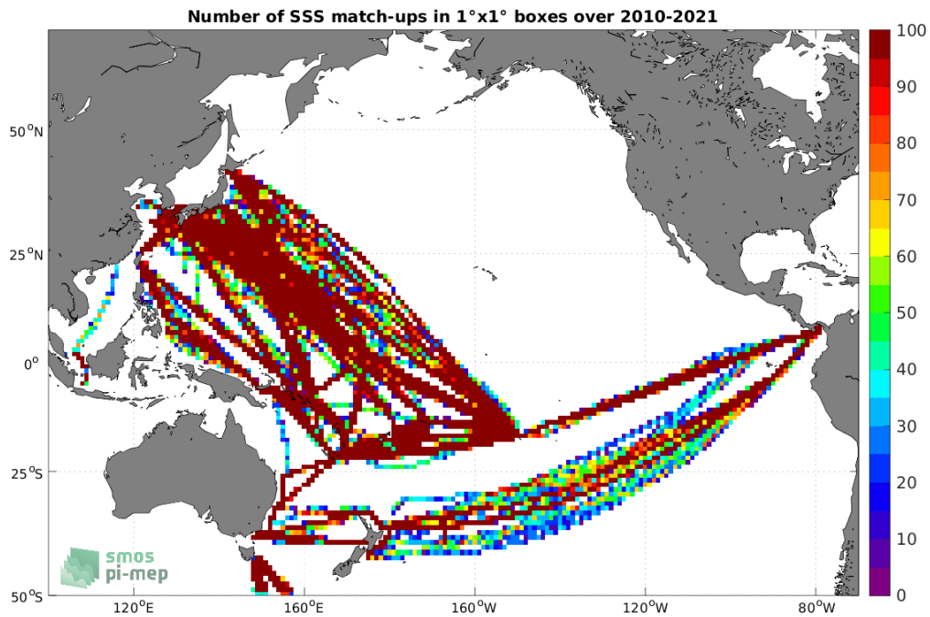
Figure 4: Number of SSS match-ups between TSG (LEGOS-DM) SSS and the SMOS SSS L4 OI v342 - Weekly (CMEMS-CATDS-LOPS) SSS product for the Pacific Ocean Pi-MEP region over 1^\circ \times 1^\circ boxes and for the full satellite product period.
