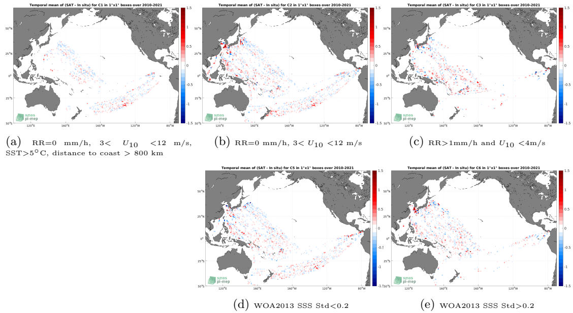
Figure 12: Temporal mean gridded over spatial boxes of size 1^\circ \times 1^\circ of \Delta SSS (SMOS SSS L4 OI v342 - Weekly (CMEMS-CATDS-LOPS) - TSG (LEGOS-DM)) for 5 different subdatasets corresponding to:RR=0 mm/h, 3 < U_{10} < 12 m/s, SST >5^\circ\text{C} , distance to coast > 800 km (a), RR=0 mm/h, 3 < U_{10} < 12 m/s (b), RR >1 mm/h and U_{10} < 4 m/s (c), WOA2013 SSS Std <0.2 (d), WOA2013 SSS Std >0.2 (e).
