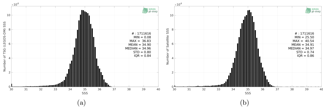
Figure 2: Histograms of SSS from TSG (LEGOS-DM) (a) and SMOS SSS L4 OI v342 - Weekly (CMEMS-CATDS-LOPS) (b) considering all match-up pairs per bins of 0.1 over the Pacific Ocean Pi-MEP region and for the full satellite product period.
