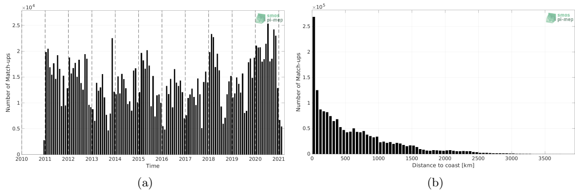
Figure 1: Number of match-ups between TSG (LEGOS-DM) and SMOS SSS L4 OI v342 - Weekly (CMEMS-CATDS-LOPS) SSS as a function of time (a) and as function of the distance to coast (b) over the Pacific Ocean Pi-MEP region and for the full satellite product period.
