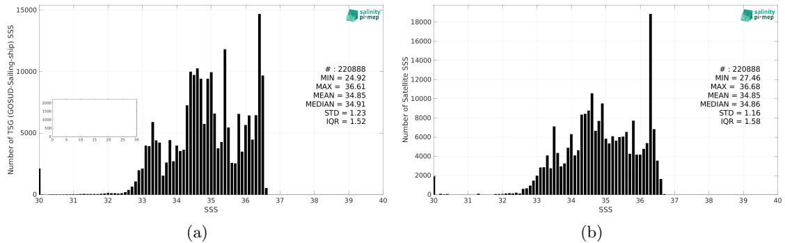
Figure 2: Histograms of SSS from TSG (GOSUD-Sailing-ship) (a) and SMOS SSS L4 OI v342 - Weekly (CMEMS-CATDS-LOPS) (b) considering all match-up pairs per bins of 0.1 over the Pacific Ocean Pi-MEP region and for the full satellite product period.
