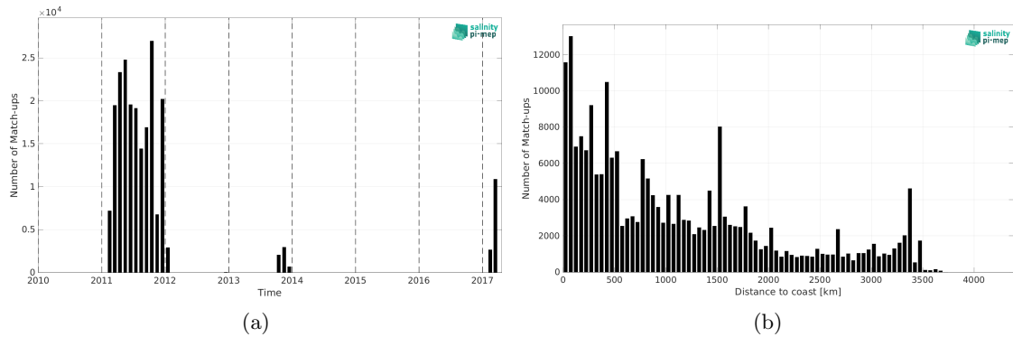
Figure 1: Number of match-ups between TSG (GOSUD-Sailing-ship) and SMOS SSS L4 OI v342 - Weekly (CMEMS-CATDS-LOPS) SSS as a function of time (a) and as function of the distance to coast (b) over the Pacific Ocean Pi-MEP region and for the full satellite product period.
