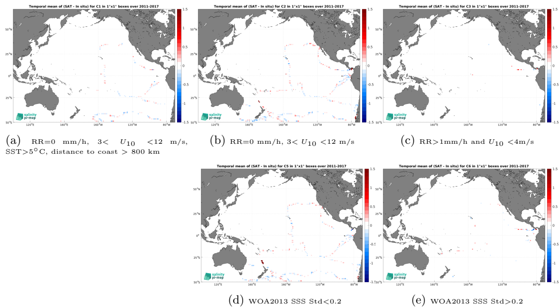
Figure 12: Temporal mean gridded over spatial boxes of size 1^\circ \times 1^\circ of \Delta SSS (SMOS SSS L4 OI v342 - Weekly (CMEMS-CATDS-LOPS) - TSG (GOSUD-Sailing-ship)) for 5 different sub-datasets corresponding to:RR=0 mm/h, 3 < U_{10} < 12 m/s, SST >5^\circ\text{C} , distance to coast > 800 km (a), RR=0 mm/h, 3 < U_{10} < 12 m/s (b), RR >1 mm/h and U_{10} < 4 m/s (c), WOA2013 SSS Std <0.2 (d), WOA2013 SSS Std >0.2 (e).
