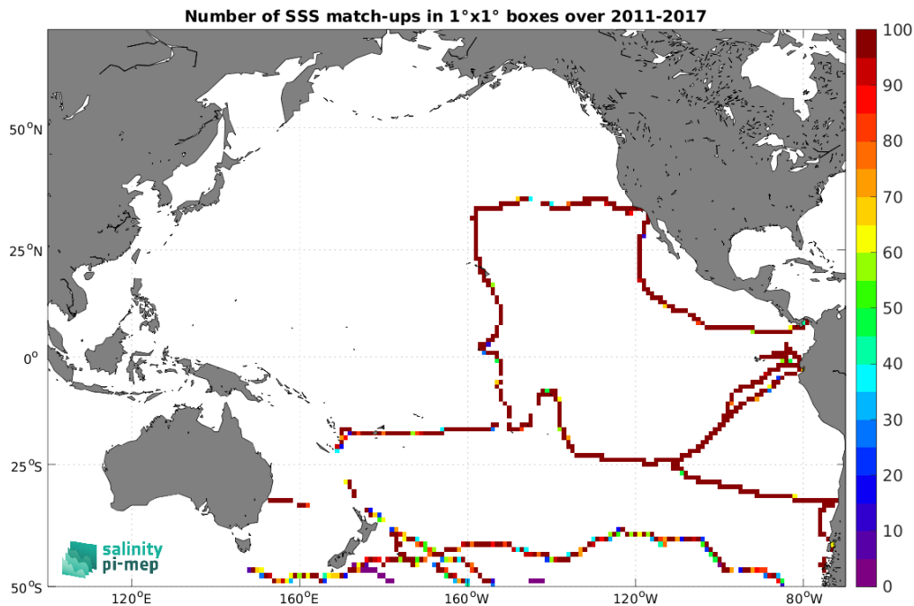
Figure 4: Number of SSS match-ups between TSG (GOSUD-Sailing-ship) SSS and the SMOS SSS L4 OI v342 - Weekly (CMEMS-CATDS-LOPS) SSS product for the Pacific Ocean Pi-MEP region over 1^\circ \times 1^\circ boxes and for the full satellite product period.
