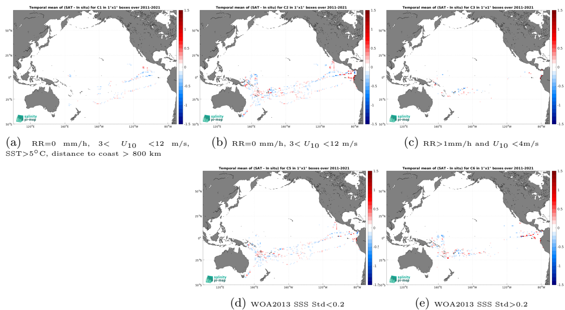
Figure 12: Temporal mean gridded over spatial boxes of size 1^\circ \times 1^\circ of \Delta\text{SSS} (SMOS SSS L4 OI v342 - Weekly (CMEMS-CATDS-LOPS) - TSG (GOSUD-Research-vessel)) for 5 different subdatasets corresponding to:RR=0 mm/h, 3 < U_{10} < 12 m/s, SST >5^\circ\text{C} , distance to coast > 800 km (a), RR=0 mm/h, 3 < U_{10} < 12 m/s (b), RR >1 mm/h and U_{10} < 4 m/s (c), WOA2013 SSS Std <0.2 (d), WOA2013 SSS Std >0.2 (e).
