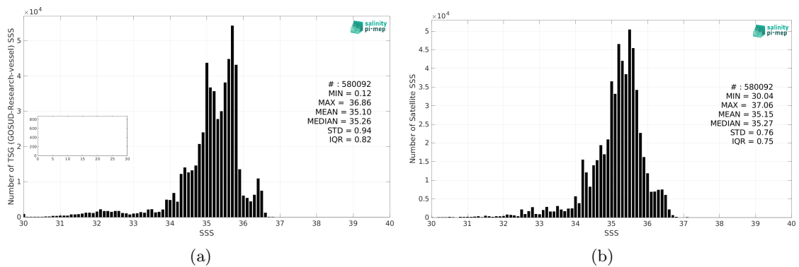
Figure 2: Histograms of SSS from TSG (GOSUD-Research-vessel) (a) and SMOS SSS L4 OI v342 - Weekly (CMEMS-CATDS-LOPS) (b) considering all match-up pairs per bins of 0.1 over the Pacific Ocean Pi-MEP region and for the full satellite product period.
