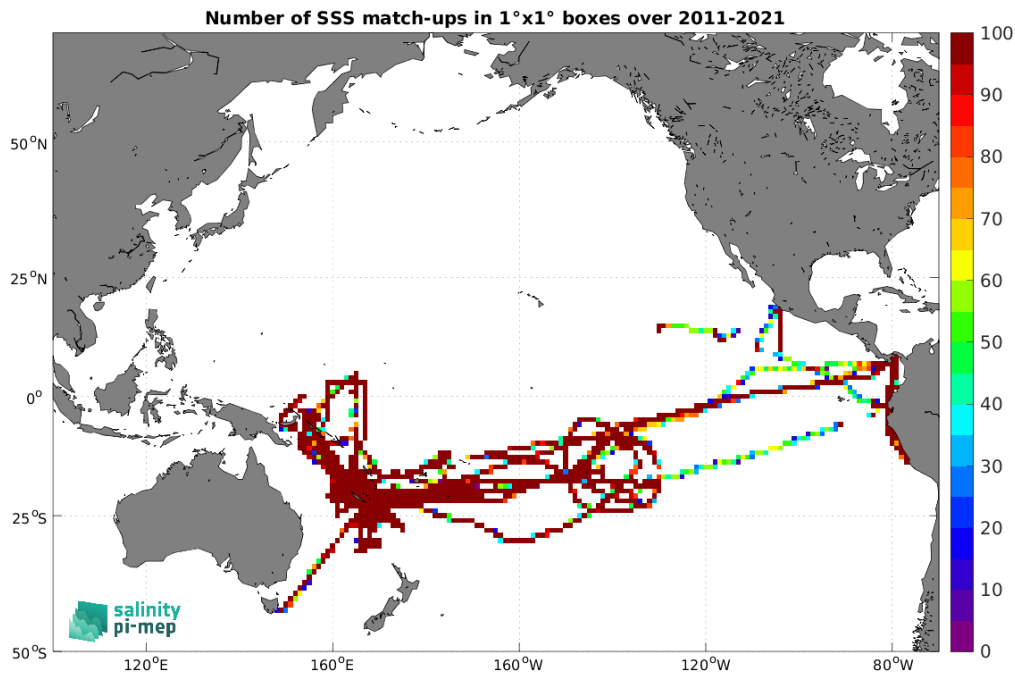
Figure 4: Number of SSS match-ups between TSG (GOSUD-Research-vessel) SSS and the SMOS SSS L4 OI v342 - Weekly (CMEMS-CATDS-LOPS) SSS product for the Pacific Ocean Pi-MEP region over 1^\circ \times 1^\circ boxes and for the full satellite product period.
