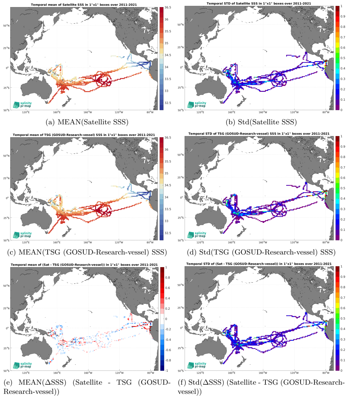
Figure 6: Temporal mean (left) and Std (right) of SSS from SMOS SSS L4 OI v342 - Weekly (CMEMS-CATDS-LOPS) (top), TSG (GOSUD-Research-vessel) (middle), and of \Delta SSS (Satellite - TSG (GOSUD-Research-vessel)). Only match-up pairs are used to generate these maps.
