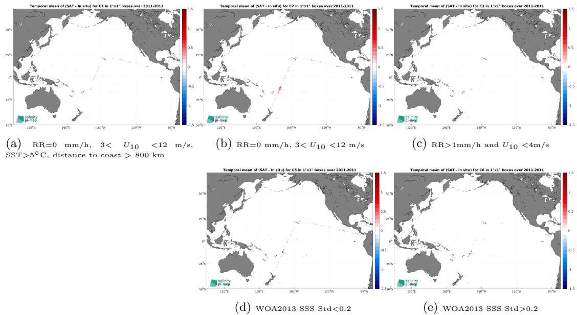
Figure 12: Temporal mean gridded over spatial boxes of size 1^\circ \times 1^\circ of \Delta SSS (SMOS SSS L4 OI v342 - Weekly (CMEMS-CATDS-LOPS) - TSG (CSIC-UTM)) for 5 different subdatasets corresponding to:RR=0 mm/h, 3 < U_{10} < 12 m/s, SST >5^\circ\text{C} , distance to coast > 800 km (a), RR=0 mm/h, 3 < U_{10} < 12 m/s (b), RR >1 mm/h and U_{10} < 4 m/s (c), WOA2013 SSS Std <0.2 (d), WOA2013 SSS Std >0.2 (e).
