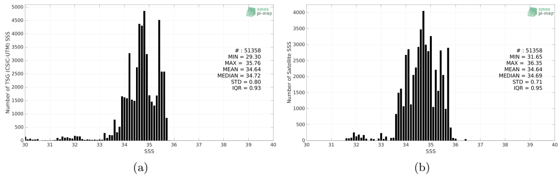
Figure 2: Histograms of SSS from TSG (CSIC-UTM) (a) and SMOS SSS L4 OI v342 - Weekly (CMEMS-CATDS-LOPS) (b) considering all match-up pairs per bins of 0.1 over the Pacific Ocean Pi-MEP region and for the full satellite product period.
