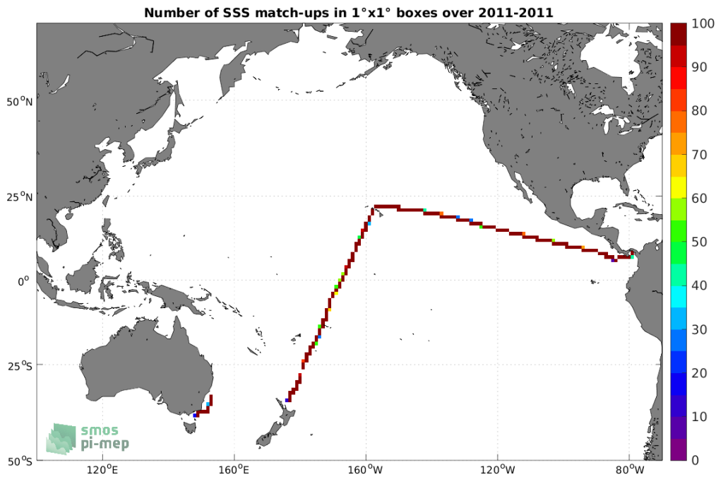
Figure 4: Number of SSS match-ups between TSG (CSIC-UTM) SSS and the SMOS SSS L4 OI v342 - Weekly (CMEMS-CATDS-LOPS) SSS product for the Pacific Ocean Pi-MEP region over 1^\circ \times 1^\circ boxes and for the full satellite product period.
