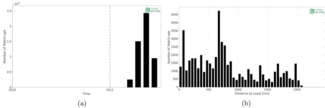
Figure 1: Number of match-ups between TSG (CSIC-UTM) and SMOS SSS L4 OI v342 - Weekly (CMEMS-CATDS-LOPS) SSS as a function of time (a) and as function of the distance to coast (b) over the Pacific Ocean Pi-MEP region and for the full satellite product period.
