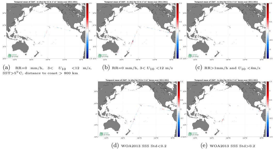
Figure 12: Temporal mean gridded over spatial boxes of size 1^{\circ}\times 1^{\circ} of \Delta\text{SSS} (SMOS SSS L4 OI v342 - Weekly (CMEMS-CATDS-LOPS) - TSG (CSIC-UTM)) for 5 different subdatasets corresponding to:RR=0 mm/h, 3 < U_{10} < 12 m/s, SST >5^{\circ}\text{C} , distance to coast > 800 km (a), RR=0 mm/h, 3 < U_{10} < 12 m/s (b), RR >1 mm/h and U_{10} < 4 m/s (c), WOA2013 SSS Std <0.2 (d), WOA2013 SSS Std >0.2 (e).
