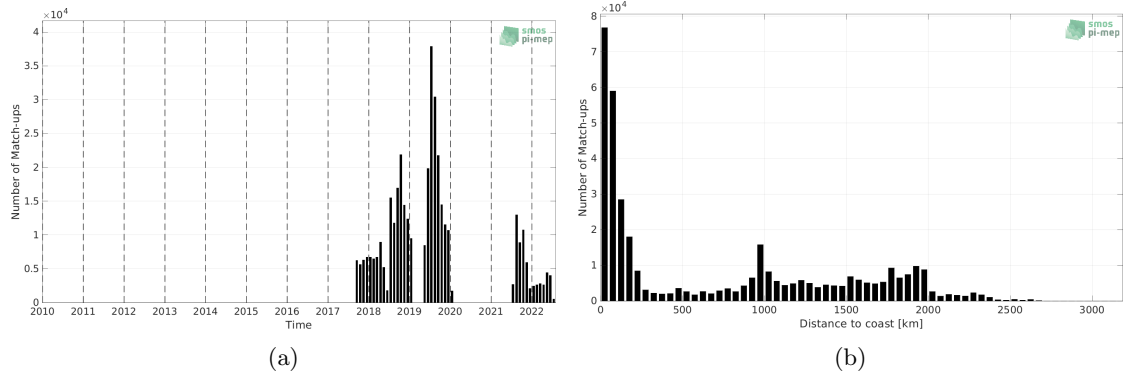
Figure 1: Number of match-ups between Saildrone and SMOS SSS L4 OI v342 - Weekly (CMEMS-CATDS-LOPS) SSS as a function of time (a) and as function of the distance to coast (b) over the Pacific Ocean Pi-MEP region and for the full satellite product period.
