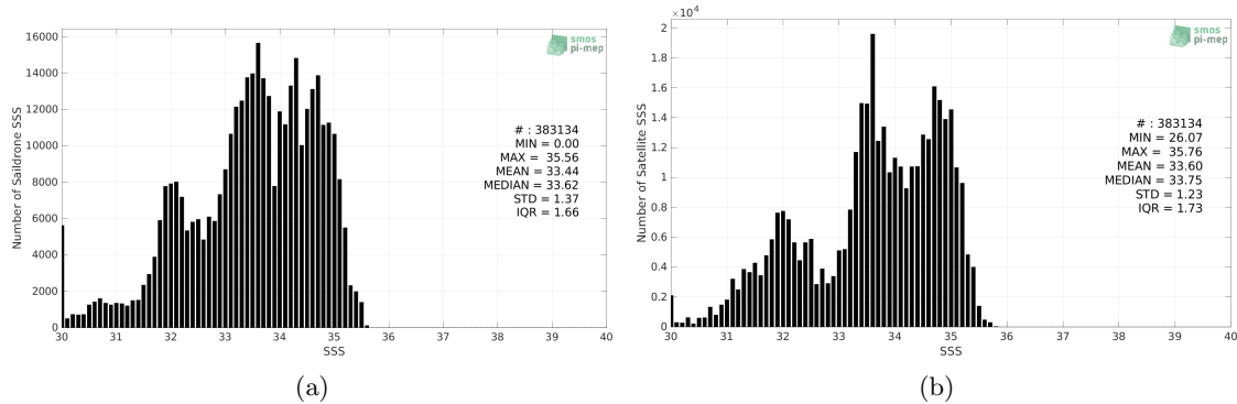
Figure 2: Histograms of SSS from Saildrone (a) and SMOS SSS L4 OI v342 - Weekly (CMEMS-CATDS-LOPS) (b) considering all match-up pairs per bins of 0.1 over the Pacific Ocean Pi-MEP region and for the full satellite product period.
