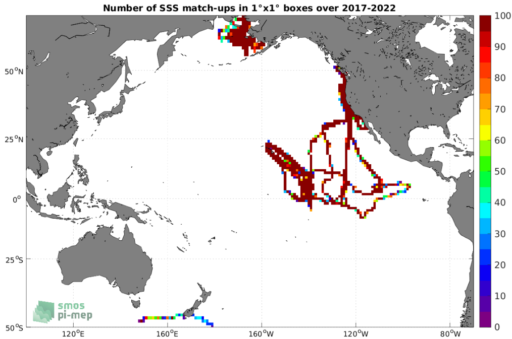
Figure 4: Number of SSS match-ups between Saildrone SSS and the SMOS SSS L4 OI v342 - Weekly (CMEMS-CATDS-LOPS) SSS product for the Pacific Ocean Pi-MEP region over 1°x1° boxes and for the full satellite product period.
