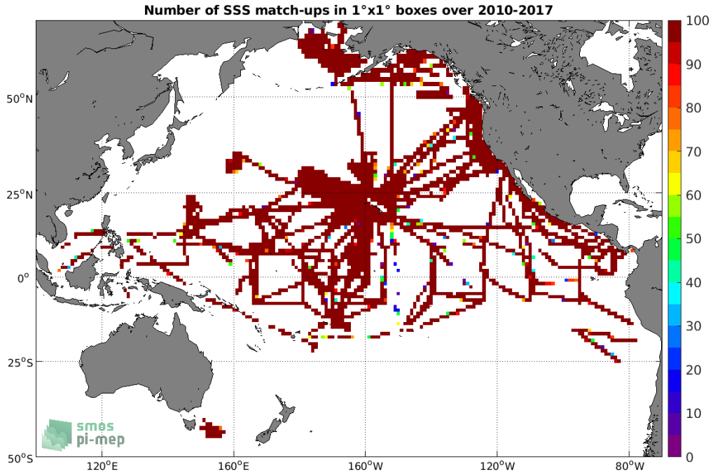
Figure 4: Number of SSS match-ups between TSG (SAMOS) SSS and the SMOS L4 v2 Weekly (CATDS-CECOS-IFREMER) SSS product for the Pacific Ocean Pi-MEP region over 1^\circ \times 1^\circ boxes and for the full satellite product period.
