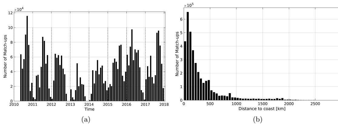
Figure 1: Number of match-ups between TSG-SAMOS and SMOS-L4-CATDS-CECOS-IFREMER-V2-WEEKLY-0.5DEG SSS as a function of time (a) and as function of the distance to coast (b) over the Pacific Ocean Pi-MEP region and for the full satellite product period.
