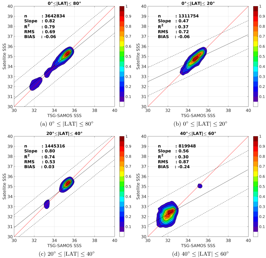
Figure 9: Contour maps of the concentration of SMOS-L4-CATDS-CECOS-IFREMER-V2-WEEKLY-0.5DEG SSS (y-axis) versus TSG-SAMOS SSS (x-axis) at match-up pairs for different latitude bands. For each plot, the red line shows x=y . The black thin and dashed lines indicate a linear fit through the data cloud and the \pm 95\% confidence levels, respectively. The number match-up pairs n , the slope and R^2 coefficient of the linear fit, the root mean square (RMS) and the mean bias between satellite and in situ data are indicated for each latitude band in each plots.
