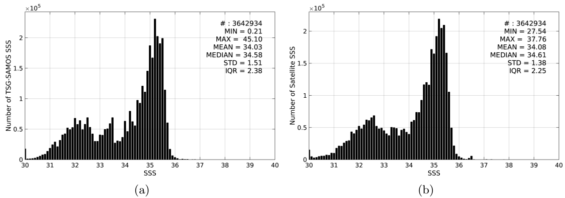
Figure 2: Histograms of SSS from TSG-SAMOS (a) and SMOS-L4-CATDS-CECOS-IFREMER-V2-WEEKLY-0.5DEG (b) considering all match-up pairs per bins of 0.1 over the Pacific Ocean Pi-MEP region and for the full satellite product period.
