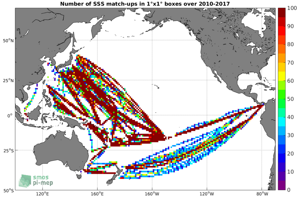
Figure 4: Number of SSS match-ups between TSG-LEGOS-DM SSS and the SMOS-L4-CATDS-CECOS-IFREMER-V2-WEEKLY-0.5DEG SSS product for the Pacific Ocean Pi-MEP region over 1^\circ \times 1^\circ boxes and for the full satellite product period.
