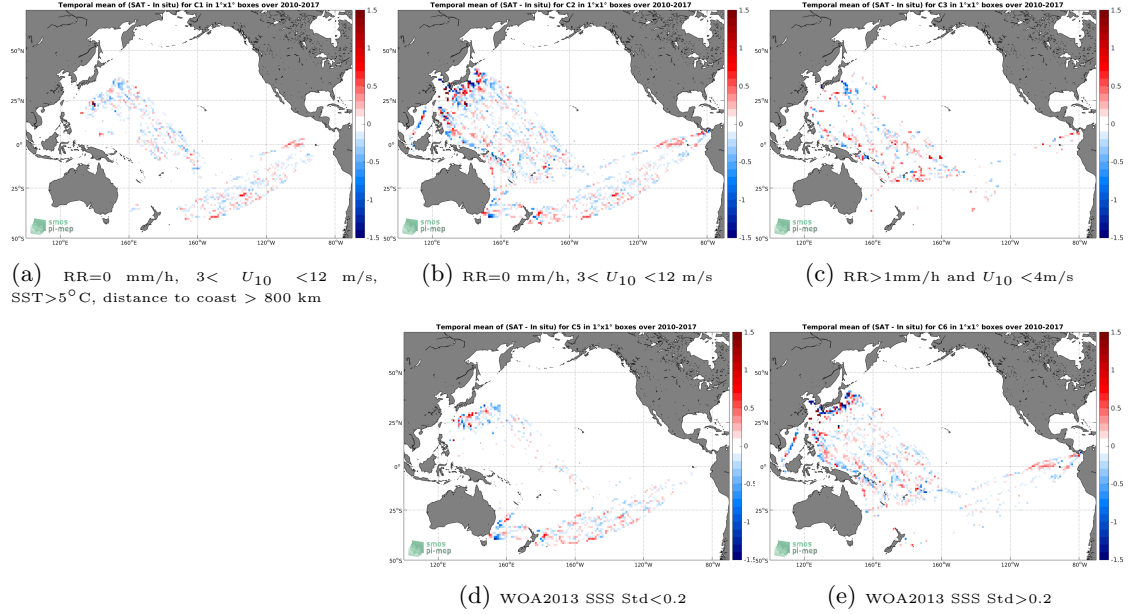
Figure 12: Temporal mean gridded over spatial boxes of size 1^\circ \times 1^\circ of \Delta SSS (SMOS-L4-CATDS-CECOS-IFREMER-V2-WEEKLY-0.5DEG - TSG-LEGOS-DM) for 5 different subdatasets corresponding to: RR=0 mm/h, 3 < U_{10} < 12 m/s, SST > 5^\circ C , distance to coast > 800 km (a), RR=0 mm/h, 3 < U_{10} < 12 m/s (b), RR > 1 mm/h and U_{10} < 4 m/s (c), WOA2013 SSS Std < 0.2 (d), WOA2013 SSS Std > 0.2 (e).
