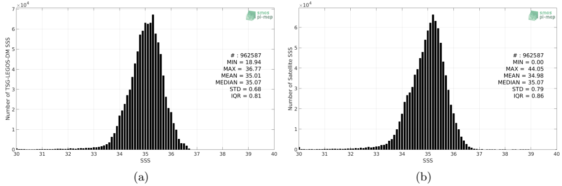
Figure 2: Histograms of SSS from TSG-LEGOS-DM (a) and SMOS-L4-CATDS-CECOS-IFREMER-V2-WEEKLY-0.5DEG (b) considering all match-up pairs per bins of 0.1 over the Pacific Ocean Pi-MEP region and for the full satellite product period.
