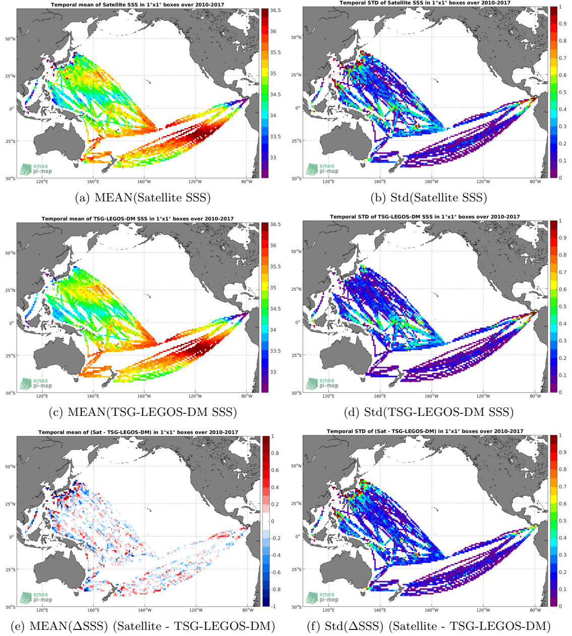
Figure 6: Temporal mean (left) and Std (right) of SSS from SMOS-L4-CATDS-CECOS-IFREMER-V2-WEEKLY-0.5DEG (top), TSG-LEGOS-DM (middle), and of \Delta SSS (Satellite - TSG-LEGOS-DM). Only match-up pairs are used to generate these maps.
