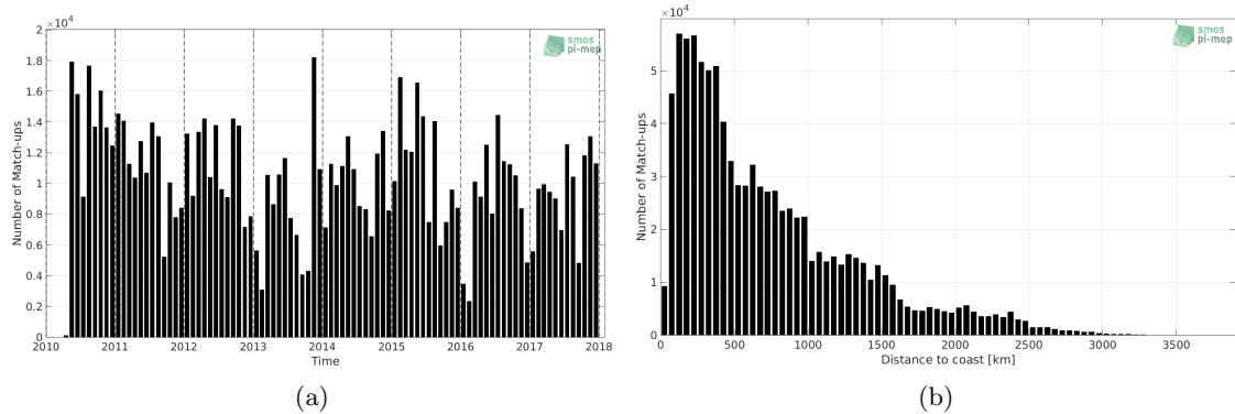
Figure 1: Number of match-ups between TSG-LEGOS-DM and SMOS-L4-CATDS-CECOS-IFREMER-V2-WEEKLY-0.5DEG SSS as a function of time (a) and as function of the distance to coast (b) over the Pacific Ocean Pi-MEP region and for the full satellite product period.
