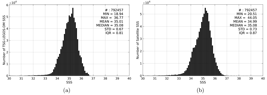
Figure 2: Histograms of SSS from TSG-LEGOS-DM (a) and SMOS-L4-CATDS-CECOS-IFREMER-V2-WEEKLY-0.5DEG (b) considering all match-up pairs per bins of 0.1 over the Pacific Ocean Pi-MEP region and for the full satellite product period.
