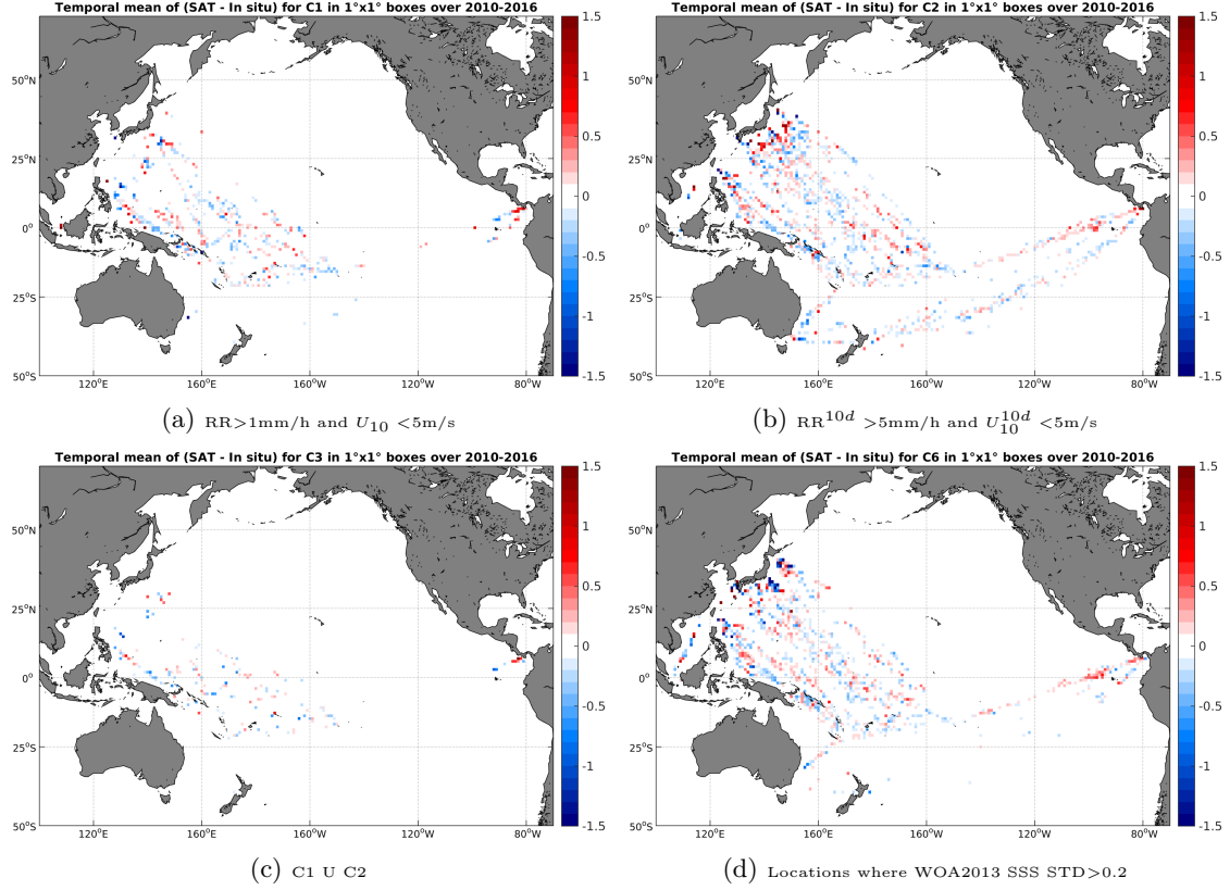
Figure 12: Temporal mean gridded over spatial boxes of size 1^\circ \times 1^\circ of \Delta SSS (SMOS-L4-CATDS-CECOS-IFREMER-V2-WEEKLY-0.5DEG - TSG-LEGOS-DM) for 4 different subdatasets corresponding to: RR > 1mm/h and U_{10} < 5 m/s (a), RR^{10d} > 5 mm/h and U_{10}^{10d} < 5 m/s (b), C1 U C2 (c), Locations where WOA2013 SSS STD > 0.2 (d).
