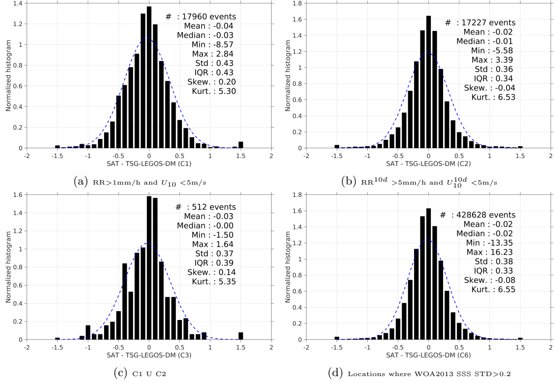
Figure 13: Normalized histogram of \Delta SSS (SMOS-L4-CATDS-CECOS-IFREMER-V2-WEEKLY-0.5DEG - TSG-LEGOS-DM) for 6 different subdatasets corresponding to: RR>1mm/h and U_{10} < 5\text{m/s} (a), RR^{10d} > 5\text{mm/h} and U_{10}^{10d} < 5\text{m/s} (b), C1 U C2 (c), Locations where WOA2013 SSS STD>0.2 (d).
