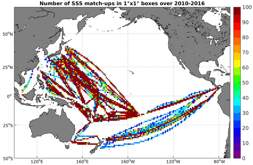
Figure 4: Number of SSS match-ups between TSG-LEGOS-DM SSS and the SMOS-L4-CATDS-CECOS-IFREMER-V2-WEEKLY-0.5DEG SSS product for the Pacific Ocean Pi-MEP region over 1^\circ \times 1^\circ boxes and for the full satellite product period.
