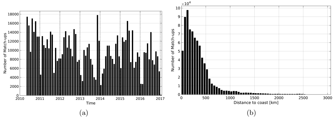
Figure 1: Number of match-ups between TSG-LEGOS-DM and SMOS-L4-CATDS-CECOS-IFREMER-V2-WEEKLY-0.5DEG SSS as a function of time (a) and as function of the distance to coast (b) over the Pacific Ocean Pi-MEP region and for the full satellite product period.
