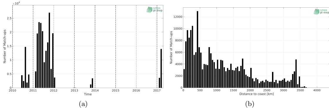
Figure 1: Number of match-ups between TSG (GOSUD-Sailing-ship) and SMOS L4 v2 Weekly (CATDS-CECOS-IFREMER) SSS as a function of time (a) and as function of the distance to coast (b) over the Pacific Ocean Pi-MEP region and for the full satellite product period.
