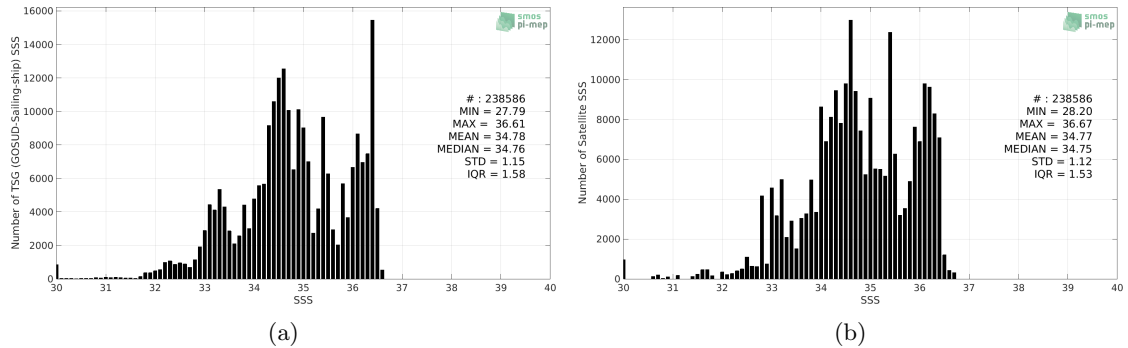
Figure 2: Histograms of SSS from TSG (GOSUD-Sailing-ship) (a) and SMOS L4 v2 Weekly (CATDS-CECOS-IFREMER) (b) considering all match-up pairs per bins of 0.1 over the Pacific Ocean Pi-MEP region and for the full satellite product period.
