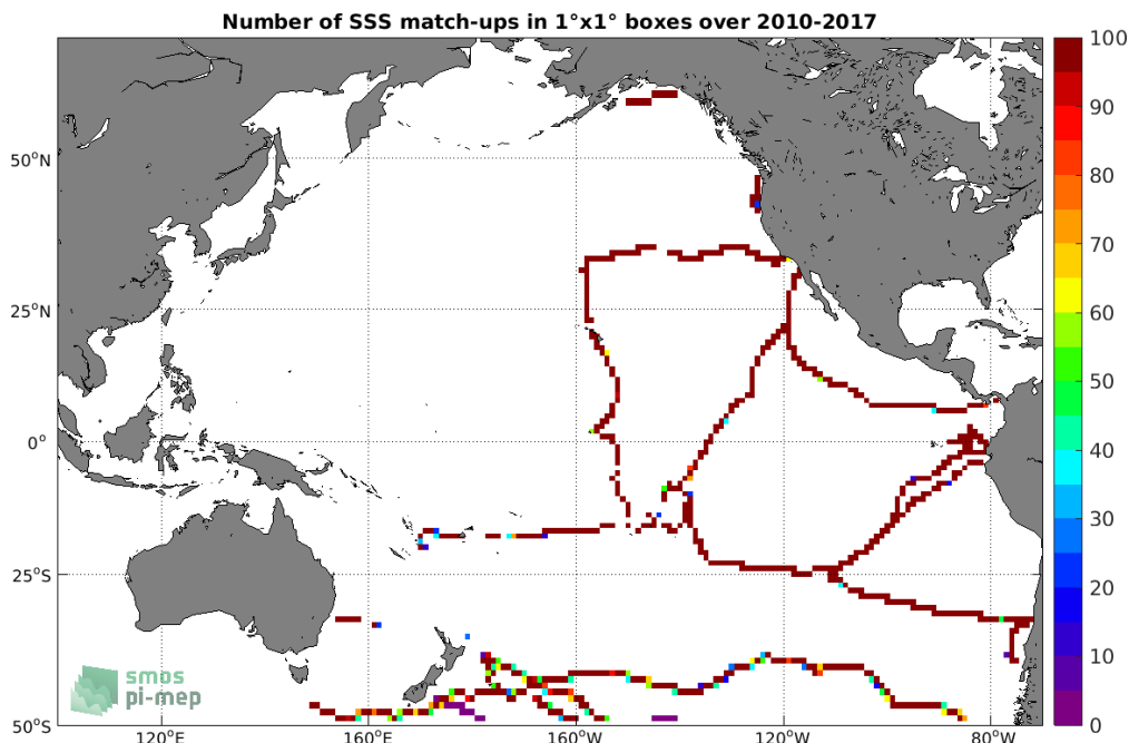
Figure 4: Number of SSS match-ups between TSG (GOSUD-Sailing-ship) SSS and the SMOS L4 v2 Weekly (CATDS-CECOS-IFREMER) SSS product for the Pacific Ocean Pi-MEP region over 1°x1° boxes and for the full satellite product period.
