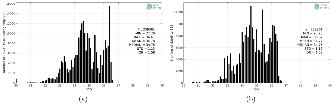
Figure 2: Histograms of SSS from TSG-GOSUD-Sailing-ship (a) and SMOS-L4-CATDS-CECOS-IFREMER-V2-WEEKLY-0.5DEG (b) considering all match-up pairs per bins of 0.1 over the Pacific Ocean Pi-MEP region and for the full satellite product period.
