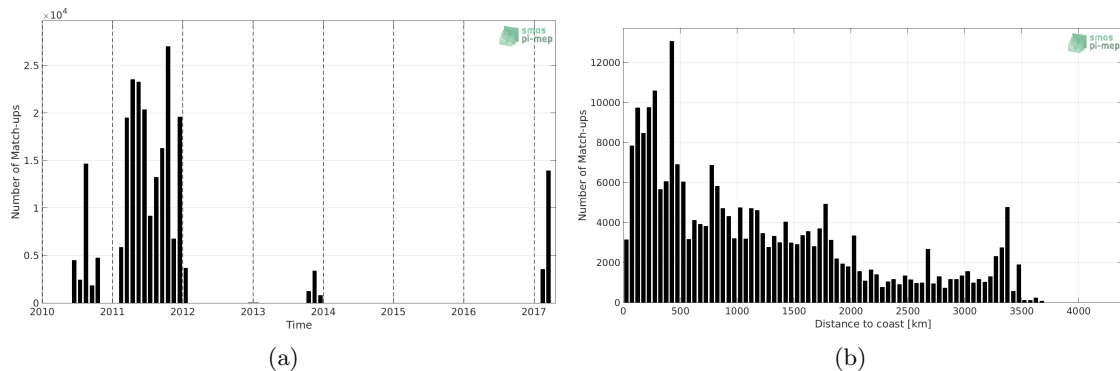
Figure 1: Number of match-ups between TSG-GOSUD-Sailing-ship and SMOS-L4-CATDS-CECOS-IFREMER-V2-WEEKLY-0.5DEG SSS as a function of time (a) and as function of the distance to coast (b) over the Pacific Ocean Pi-MEP region and for the full satellite product period.
