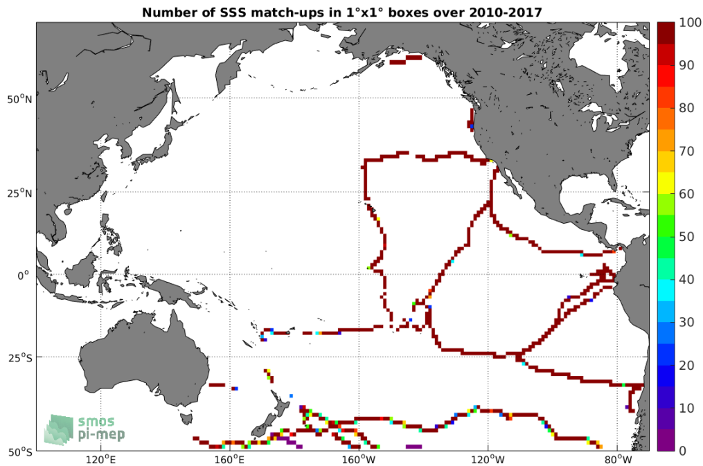
Figure 4: Number of SSS match-ups between TSG-GOSUD-Sailing-ship SSS and the SMOS-L4-CATDS-CECOS-IFREMER-V2-WEEKLY-0.5DEG SSS product for the Pacific Ocean Pi-MEP region over 1^\circ \times 1^\circ boxes and for the full satellite product period.
