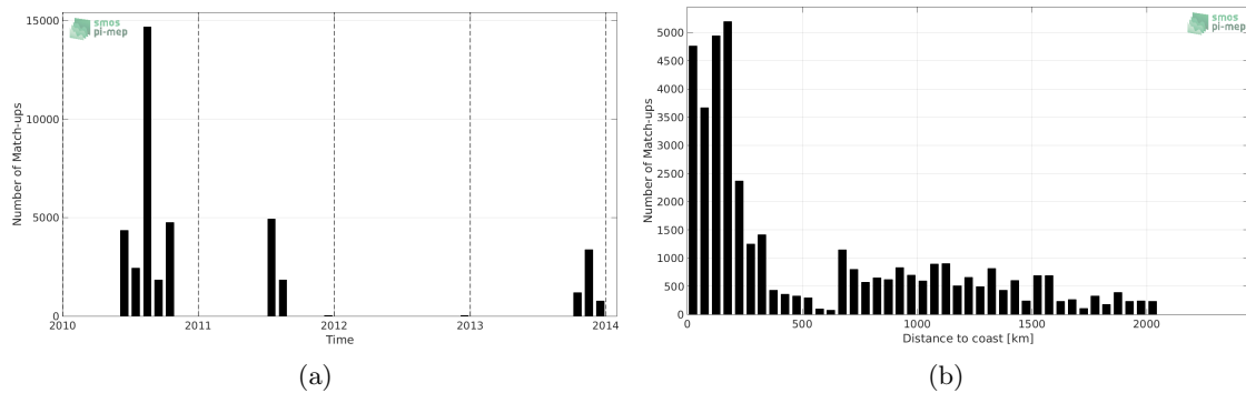
Figure 1: Number of match-ups between TSG-GOSUD-Sailing-ship and SMOS-L4-CATDS-CECOS-IFREMER-V2-WEEKLY-0.5DEG SSS as a function of time (a) and as function of the distance to coast (b) over the Pacific Ocean Pi-MEP region and for the full satellite product period.
