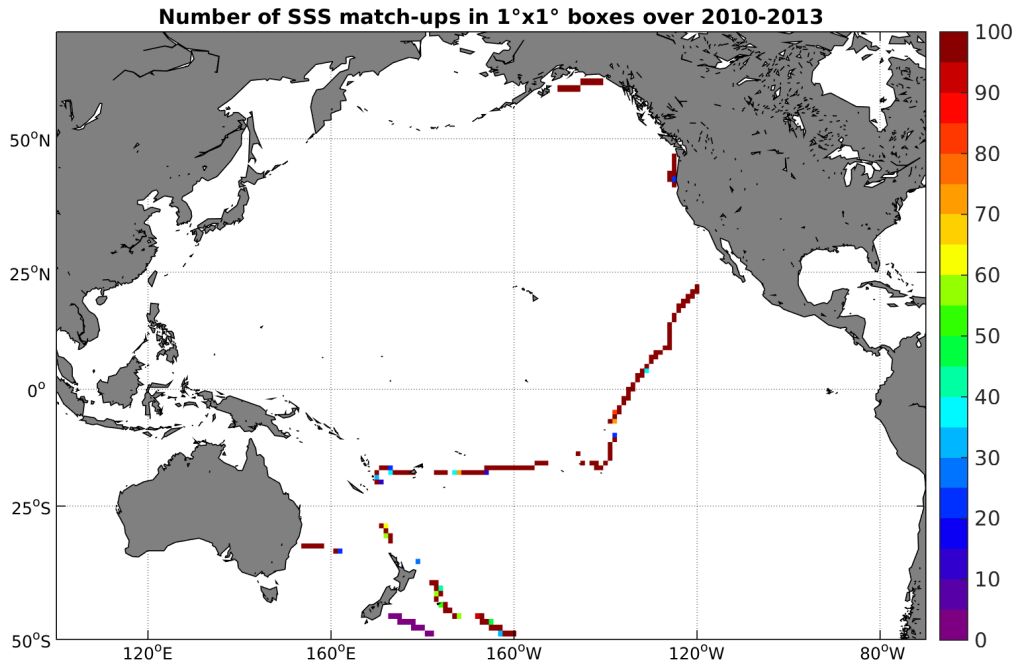
Figure 4: Number of SSS match-ups between TSG-GOSUD-Sailing-ship SSS and the SMOS-L4-CATDS-CECOS-IFREMER-V2-WEEKLY-0.5DEG SSS product for the Pacific Ocean Pi-MEP region over 1°x1° boxes and for the full satellite product period.
