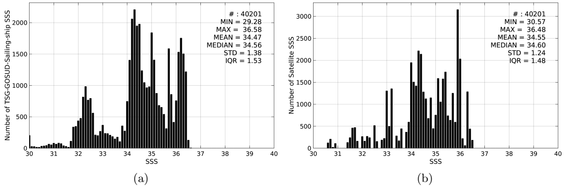
Figure 2: Histograms of SSS from TSG-GOSUD-Sailing-ship (a) and SMOS-L4-CATDS-CECOS-IFREMER-V2-WEEKLY-0.5DEG (b) considering all match-up pairs per bins of 0.1 over the Pacific Ocean Pi-MEP region and for the full satellite product period.
