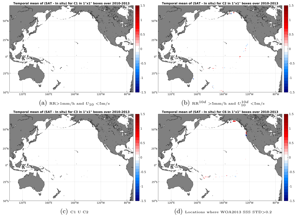
Figure 12: Temporal mean gridded over spatial boxes of size 1^\circ \times 1^\circ of \Delta SSS (SMOS-L4-CATDS-CECOS-IFREMER-V2-WEEKLY-0.5DEG - TSG-GOSUD-Sailing-ship) for 4 different subdatasets corresponding to: RR > 1\text{mm/h} and U_{10} < 5\text{m/s} (a), RR^{10d} > 5\text{mm/h} and U_{10}^{10d} < 5\text{m/s} (b), C1 U C2 (c), Locations where WOA2013 SSS STD > 0.2 (d).
