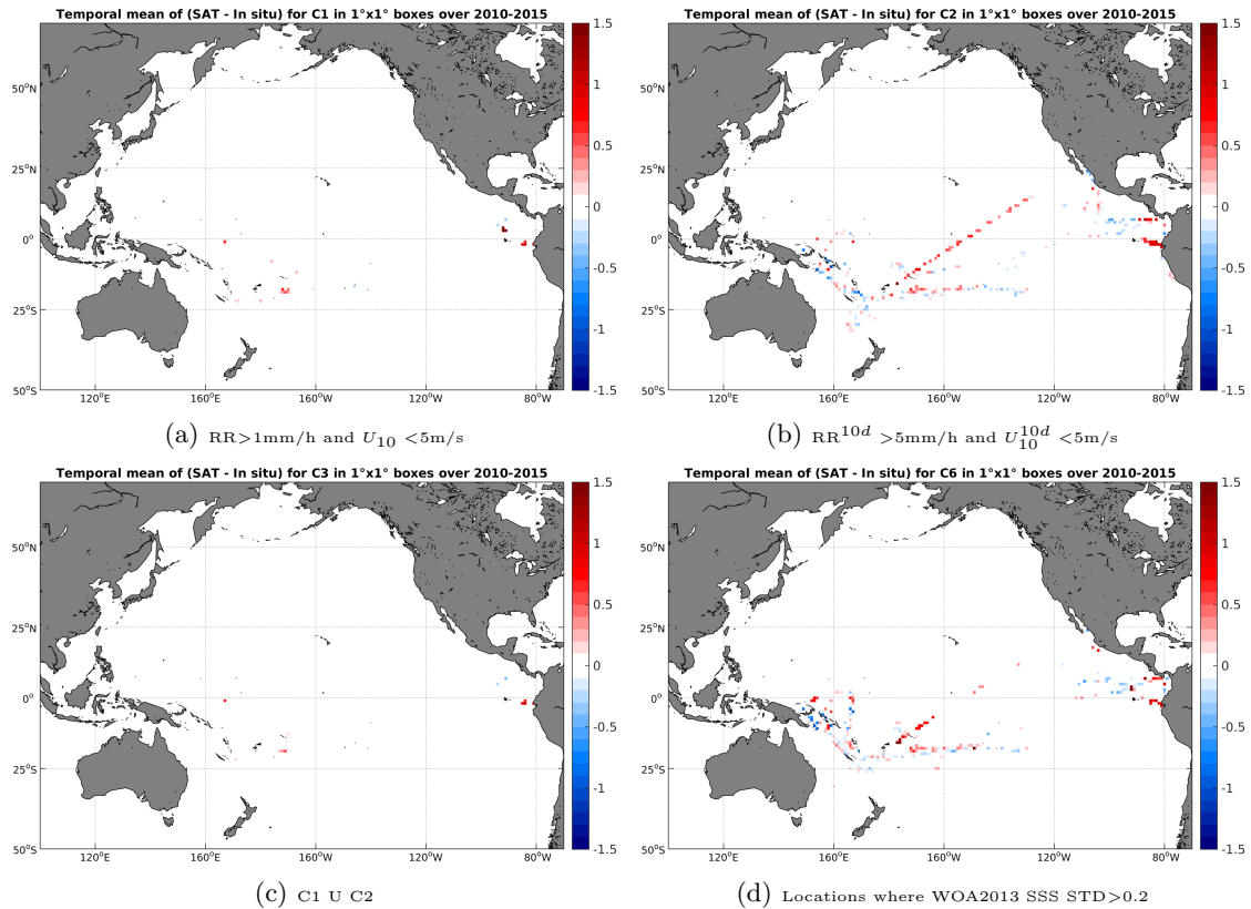
Figure 12: Temporal mean gridded over spatial boxes of size 1°x1° of \Delta SSS (SMOS-L4-CATDS-CECOS-IFREMER-V2-WEEKLY-0.5DEG - TSG-GOSUD-Research-vessel) for 4 different sub-datasets corresponding to: RR > 1mm/h and U_{10} < 5\text{m/s} (a), RR^{10d} > 5\text{mm/h} and U_{10}^{10d} < 5\text{m/s} (b), C1 U C2 (c), Locations where WOA2013 SSS STD > 0.2 (d).
