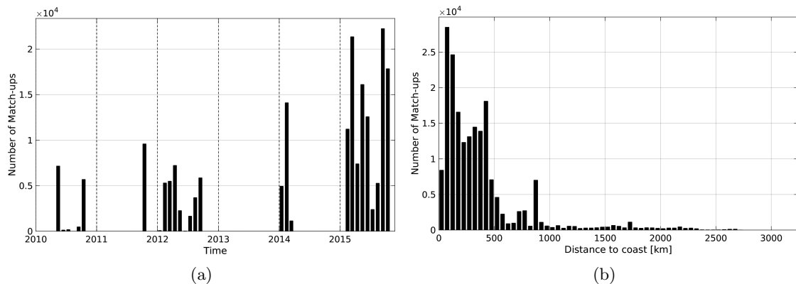
Figure 1: Number of match-ups between TSG-GOSUD-Research-vessel and SMOS-L4-CATDS-CECOS-IFREMER-V2-WEEKLY-0.5DEG SSS as a function of time (a) and as function of the distance to coast (b) over the Pacific Ocean Pi-MEP region and for the full satellite product period.
