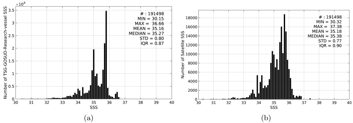
Figure 2: Histograms of SSS from TSG-GOSUD-Research-vessel (a) and SMOS-L4-CATDS-CECOS-IFREMER-V2-WEEKLY-0.5DEG (b) considering all match-up pairs per bins of 0.1 over the Pacific Ocean Pi-MEP region and for the full satellite product period.
