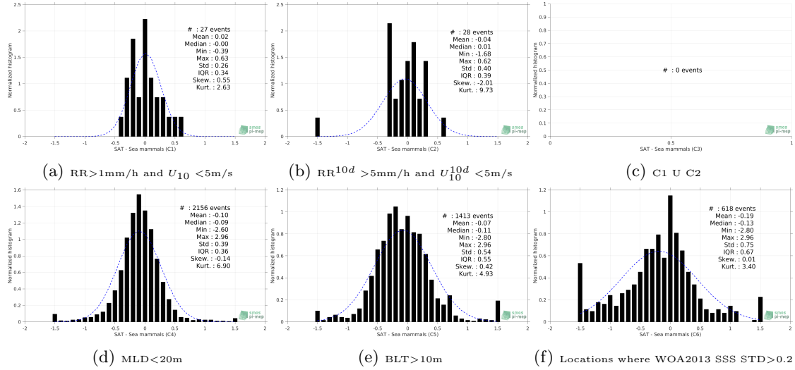
Figure 13: Normalized histogram of \Delta SSS (SMOS-L4-CATDS-CECOS-IFREMER-V2-WEEKLY-0.5DEG - Sea mammals) for 6 different subdatasets corresponding to: RR > 1\text{mm/h} and U_{10} < 5\text{m/s} (a), RR^{10d} > 5\text{mm/h} and U_{10}^{10d} < 5\text{m/s} (b), C1 \cup C2 (c), MLD < 20\text{m} (d), BLT > 10\text{m} (e), Locations where WOA2013 SSS STD > 0.2 (f).
