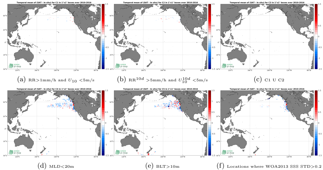
Figure 12: Temporal mean gridded over spatial boxes of size 1^\circ \times 1^\circ of \Delta\text{SSS} (SMOS-L4-CATDS-CECOS-IFREMER-V2-WEEKLY-0.5DEG - Sea mammals) for 6 different subdatasets corresponding to: RR > 1\text{mm/h} and U_{10} < 5\text{m/s} (a), RR^{10d} > 5\text{mm/h} and U_{10}^{10d} < 5\text{m/s} (b), C1 U C2 (c), \text{MLD} < 20\text{m} (d), \text{BLT} > 10\text{m} (e), Locations where WOA2013 SSS STD > 0.2 (f).
