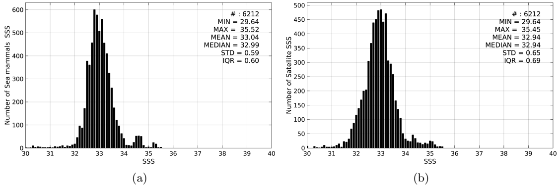
Figure 2: Histograms of SSS from Sea mammals (a) and SMOS-L4-CATDS-CECOS-IFREMER-V2-WEEKLY-0.5DEG (b) considering all match-up pairs per bins of 0.1 over the Pacific Ocean Pi-MEP region and for the full satellite product period.
