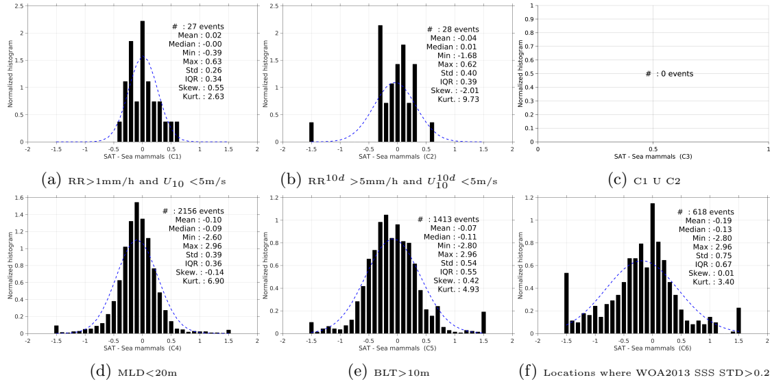
Figure 13: Normalized histogram of \Delta SSS (SMOS-L4-CATDS-CECOS-IFREMER-V2-WEEKLY-0.5DEG - Sea mammals) for 6 different subdatasets corresponding to: RR>1mm/h and U_{10} < 5\text{m/s} (a), RR^{10d} > 5\text{mm/h} and U_{10}^{10d} < 5\text{m/s} (b), C1 U C2 (c),MLD<20m (d),BLT>10m (e),Locations where WOA2013 SSS STD>0.2 (f).
