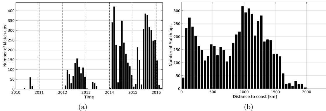
Figure 1: Number of match-ups between Sea mammals and SMOS-L4-CATDS-CECOS-IFREMER-V2-WEEKLY-0.5DEG SSS as a function of time (a) and as function of the distance to coast (b) over the Pacific Ocean Pi-MEP region and for the full satellite product period.
