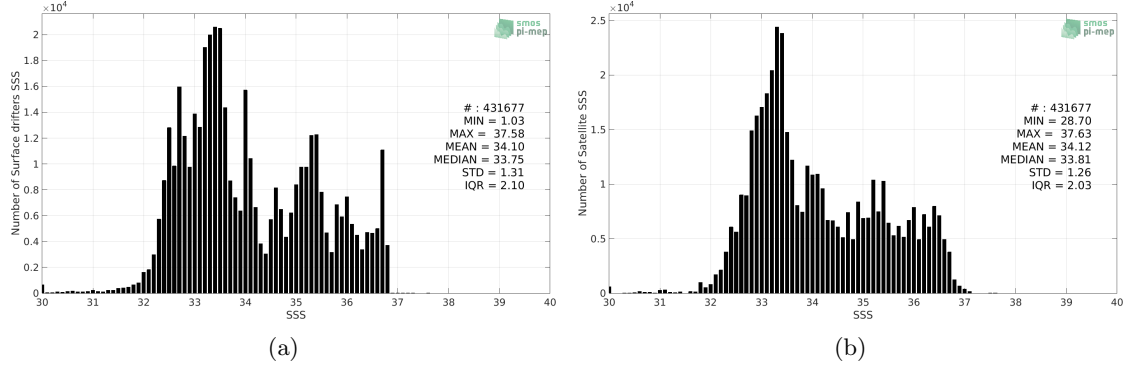
Figure 2: Histograms of SSS from Surface drifters (a) and SMOS L4 v2 Weekly (CATDS-CECOS-IFREMER) (b) considering all match-up pairs per bins of 0.1 over the Pacific Ocean Pi-MEP region and for the full satellite product period.
