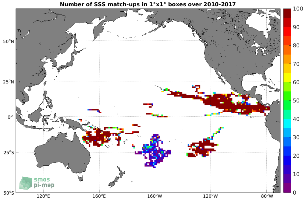
Figure 3: Number of SSS match-ups between Surface drifters SSS and the SMOS L4 v2 Weekly (CATDS-CECOS-IFREMER) SSS product for the Pacific Ocean Pi-MEP region over 1°x1° boxes and for the full satellite product period.
