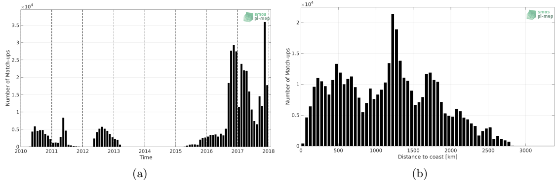
Figure 1: Number of match-ups between Surface drifters and SMOS L4 v2 Weekly (CATDS-CECOS-IFREMER) SSS as a function of time (a) and as function of the distance to coast (b) over the Pacific Ocean Pi-MEP region and for the full satellite product period.
