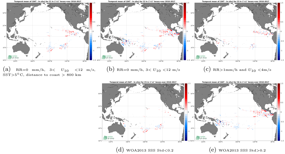
Figure 11: Temporal mean gridded over spatial boxes of size 1^{\circ}\times 1^{\circ} of \Delta\text{SSS} (SMOS L4 v2 Weekly (CATDS-CECOS-IFREMER) - Surface drifters) for 5 different subdatasets corresponding to: RR=0 mm/h, 3 < U_{10} < 12 m/s, SST >5^{\circ}\text{C} , distance to coast > 800 km (a), RR=0 mm/h, 3 < U_{10} < 12 m/s (b), RR >1 mm/h and U_{10} < 4 m/s (c), WOA2013 SSS Std <0.2 (d), WOA2013 SSS Std >0.2 (e).
