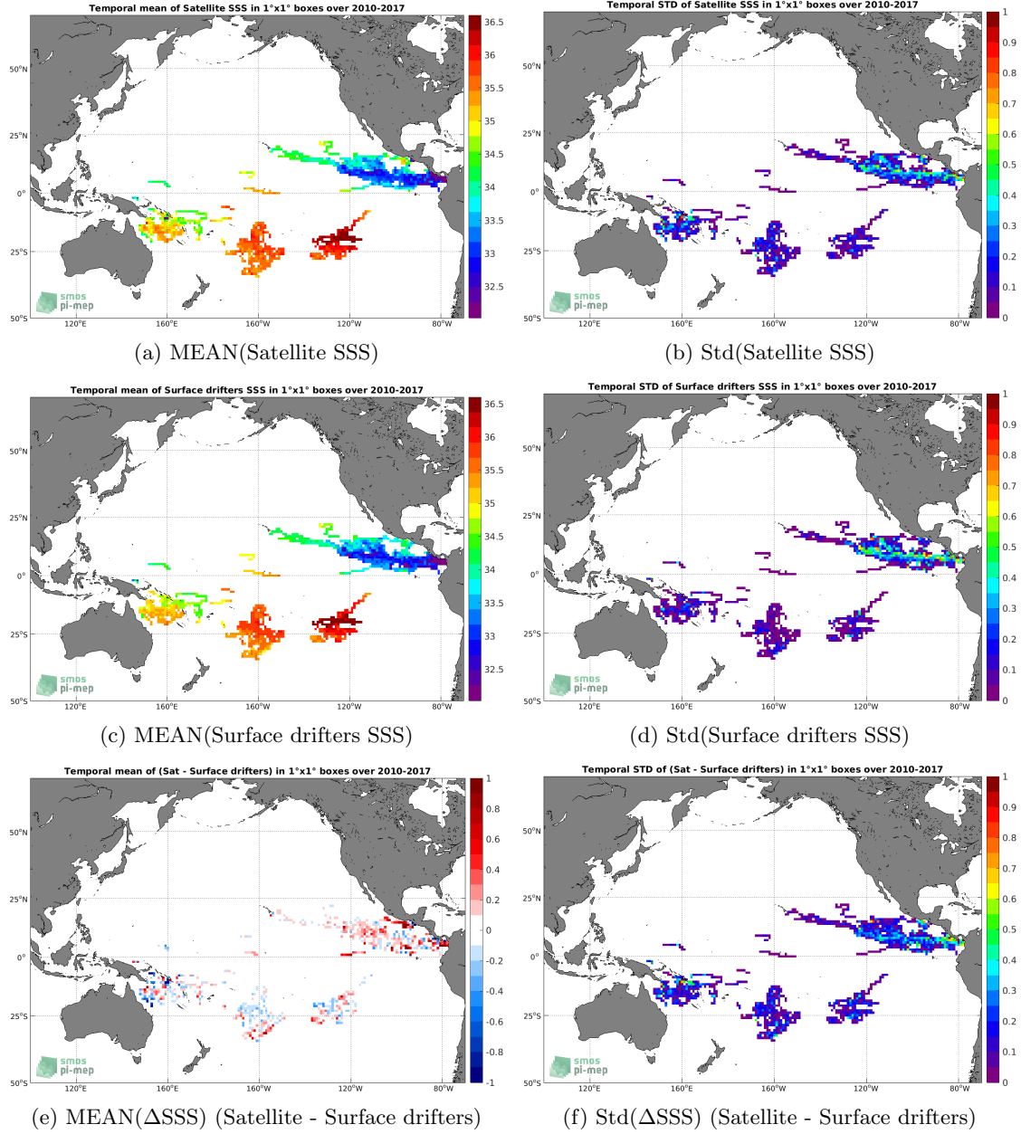
Figure 5: Temporal mean (left) and Std (right) of SSS from SMOS L4 v2 Weekly (CATDS-CECOS-IFREMER) (top), Surface drifters (middle), and of \Delta SSS (Satellite - Surface drifters). Only match-up pairs are used to generate these maps.
