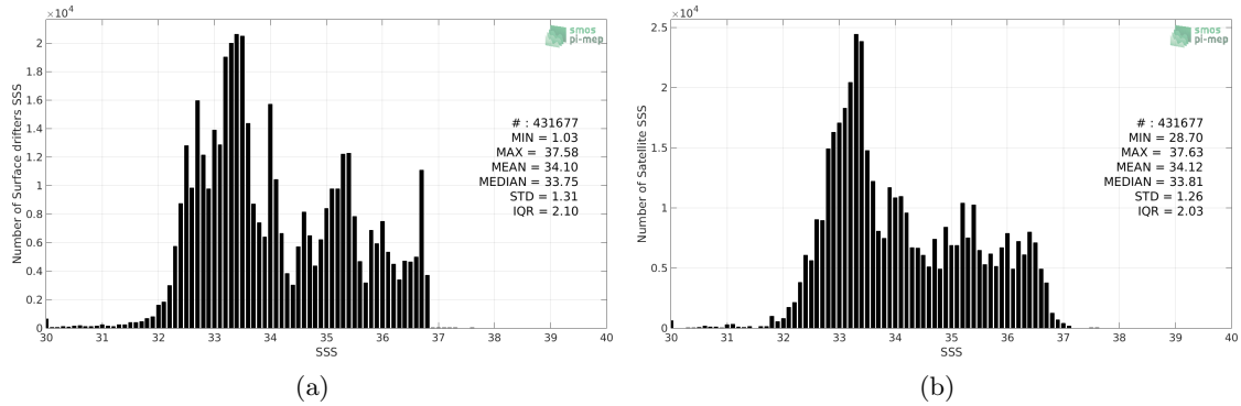
Figure 2: Histograms of SSS from Surface drifters (a) and SMOS-L4-CATDS-CECOS-IFREMER-V2-WEEKLY-0.5DEG (b) considering all match-up pairs per bins of 0.1 over the Pacific Ocean Pi-MEP region and for the full satellite product period.
