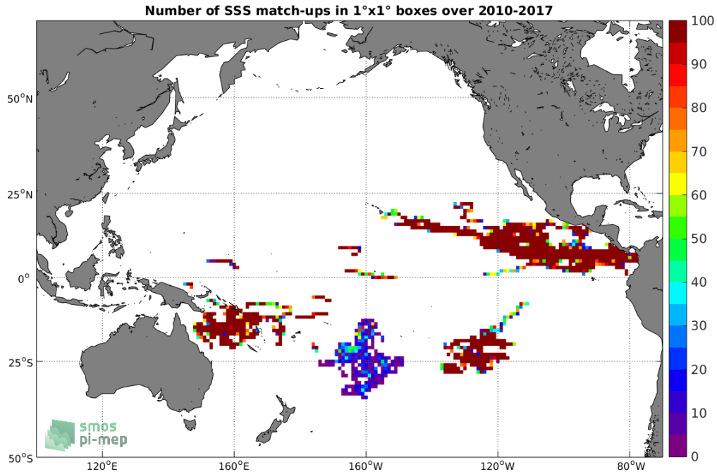
Figure 3: Number of SSS match-ups between Surface drifters SSS and the SMOS-L4-CATDS-CECOS-IFREMER-V2-WEEKLY-0.5DEG SSS product for the Pacific Ocean Pi-MEP region over 1°x1° boxes and for the full satellite product period.
