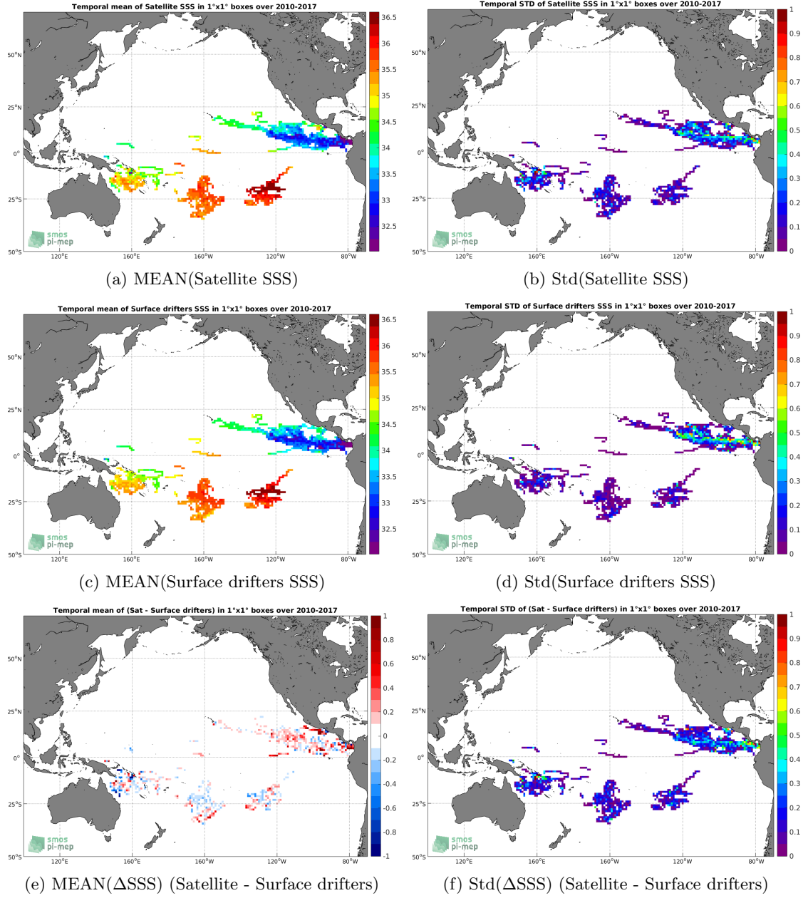
Figure 5: Temporal mean (left) and Std (right) of SSS from SMOS-L4-CATDS-CECOS-IFREMER-V2-WEEKLY-0.5DEG (top), Surface drifters (middle), and of \Delta SSS (Satellite - Surface drifters). Only match-up pairs are used to generate these maps.
