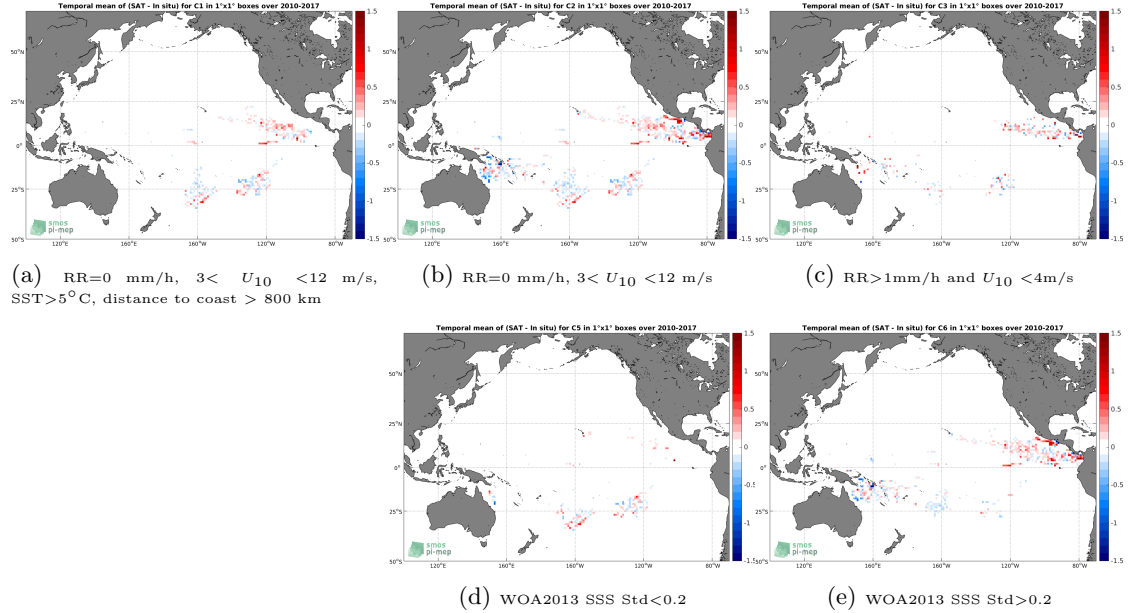
Figure 11: Temporal mean gridded over spatial boxes of size 1^{\circ}\times 1^{\circ} of \Delta\text{SSS} (SMOS-L4-CATDS-CECOS-IFREMER-V2-WEEKLY-0.5DEG - Surface drifters) for 5 different subdatasets corresponding to: RR=0 mm/h, 3 < U_{10} < 12 m/s, SST >5^{\circ}\text{C} , distance to coast > 800 km (a), RR=0 mm/h, 3 < U_{10} < 12 m/s (b), RR >1 mm/h and U_{10} < 4 m/s (c), WOA2013 SSS Std <0.2 (d), WOA2013 SSS Std >0.2 (e).
