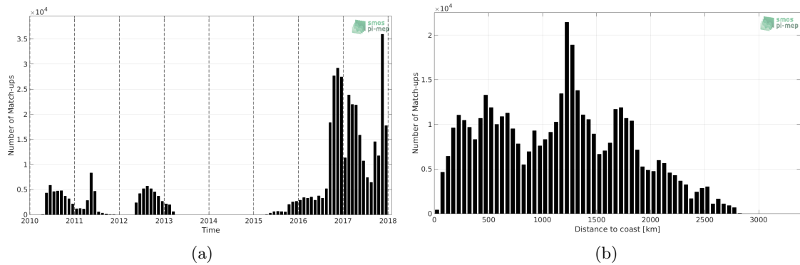
Figure 1: Number of match-ups between Surface drifters and SMOS-L4-CATDS-CECOS-IFREMER-V2-WEEKLY-0.5DEG SSS as a function of time (a) and as function of the distance to coast (b) over the Pacific Ocean Pi-MEP region and for the full satellite product period.
