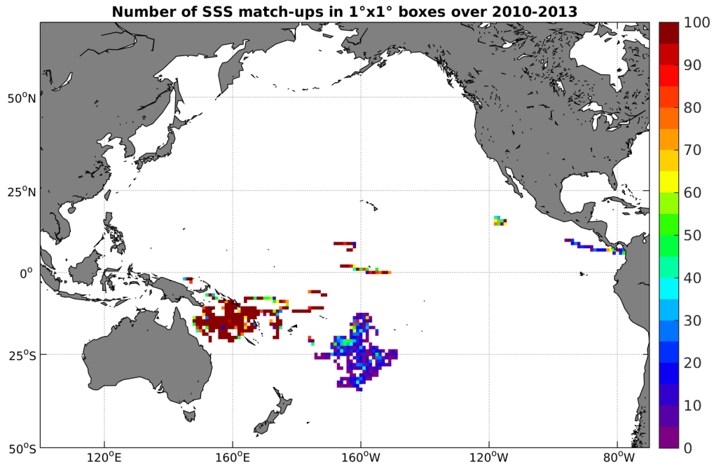
Figure 3: Number of SSS match-ups between Surface drifters SSS and the SMOS-L4-CATDS-CECOS-IFREMER-V2-WEEKLY-0.5DEG SSS product for the Pacific Ocean Pi-MEP region over 1°x1° boxes and for the full satellite product period.
