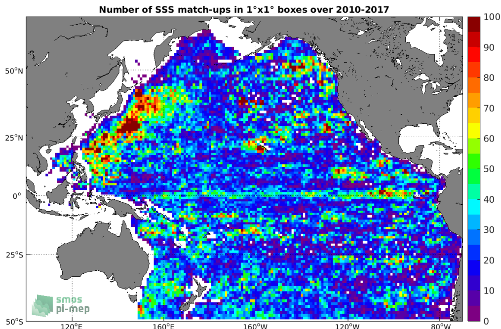
Figure 4: Number of SSS match-ups between Argo SSS and the SMOS L4 v2 Weekly (CATDS-CECOS-IFREMER) SSS product for the Pacific Ocean Pi-MEP region over 1°x1° boxes and for the full satellite product period.
