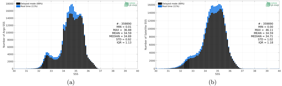
Figure 2: Histograms of SSS from Argo (a) and SMOS L4 v2 Weekly (CATDS-CECOS-IFREMER) (b) considering all match-up pairs per bins of 0.1 over the Pacific Ocean Pi-MEP region and for the full satellite product period.
