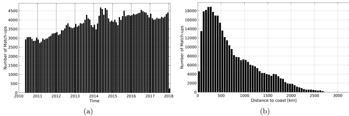
Figure 1: Number of match-ups between Argo and SMOS-L4-CATDS-CECOS-IFREMER-V2-WEEKLY-0.5DEG SSS as a function of time (a) and as function of the distance to coast (b) over the Pacific Ocean Pi-MEP region and for the full satellite product period.
