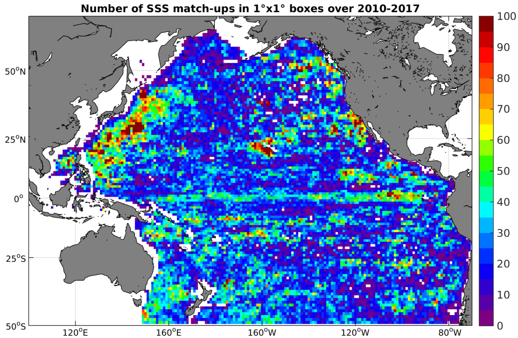
Figure 4: Number of SSS match-ups between Argo SSS and the SMOS-L4-CATDS-CECOS-IFREMER-V2-WEEKLY-0.5DEG SSS product for the Pacific Ocean Pi-MEP region over 1°x1° boxes and for the full satellite product period.
