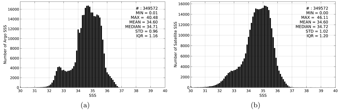
Figure 2: Histograms of SSS from Argo (a) and SMOS-L4-CATDS-CECOS-IFREMER-V2-WEEKLY-0.5DEG (b) considering all match-up pairs per bins of 0.1 over the Pacific Ocean Pi-MEP region and for the full satellite product period.
