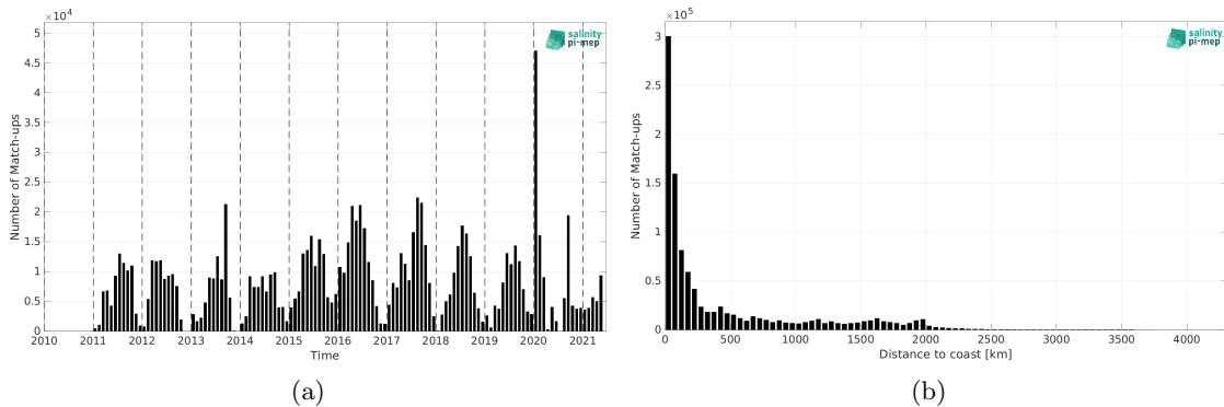
Figure 1: Number of match-ups between TSG (SAMOS) and SMOS SSS L4 v2 - Daily (BEC) SSS as a function of time (a) and as function of the distance to coast (b) over the Pacific Ocean Pi-MEP region and for the full satellite product period.
