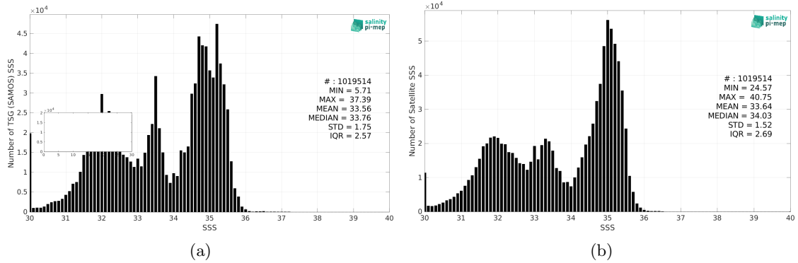
Figure 2: Histograms of SSS from TSG (SAMOS) (a) and SMOS SSS L4 v2 - Daily (BEC) (b) considering all match-up pairs per bins of 0.1 over the Pacific Ocean Pi-MEP region and for the full satellite product period.
