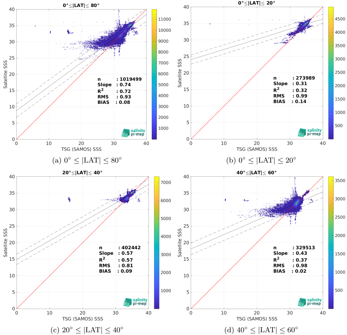
Figure 9: Contour maps of the concentration of SMOS SSS L4 v2 - Daily (BEC) SSS (y-axis) versus TSG (SAMOS) SSS (x-axis) at match-up pairs for different latitude bands. For each plot, the red line shows x=y . The black thin and dashed lines indicate a linear fit through the data cloud and the \pm 95\% confidence levels, respectively. The number match-up pairs n , the slope and R^2 coefficient of the linear fit, the root mean square (RMS) and the mean bias between satellite and in situ data are indicated for each latitude band in each plots.
