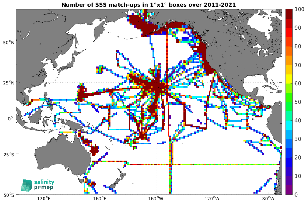
Figure 4: Number of SSS match-ups between TSG (SAMOS) SSS and the SMOS SSS L4 v2 - Daily (BEC) SSS product for the Pacific Ocean Pi-MEP region over 1^\circ \times 1^\circ boxes and for the full satellite product period.
