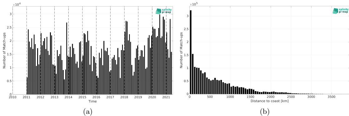
Figure 2: Number of match-ups between TSG (LEGOS-DM) and SMOS SSS L4 v2 - Daily (BEC) SSS as a function of time (a) and as function of the distance to coast (b) over the Pacific Ocean Pi-MEP region and for the full satellite product period.
