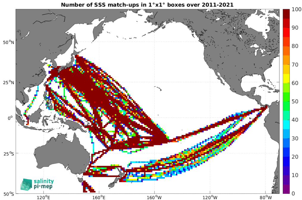
Figure 5: Number of SSS match-ups between TSG (LEGOS-DM) SSS and the SMOS SSS L4 v2 - Daily (BEC) SSS product for the Pacific Ocean Pi-MEP region over 1^\circ \times 1^\circ boxes and for the full satellite product period.
