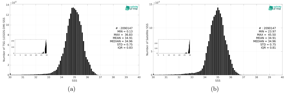
Figure 3: Histograms of SSS from TSG (LEGOS-DM) (a) and SMOS SSS L4 v2 - Daily (BEC) (b) considering all match-up pairs per bins of 0.1 over the Pacific Ocean Pi-MEP region and for the full satellite product period.
