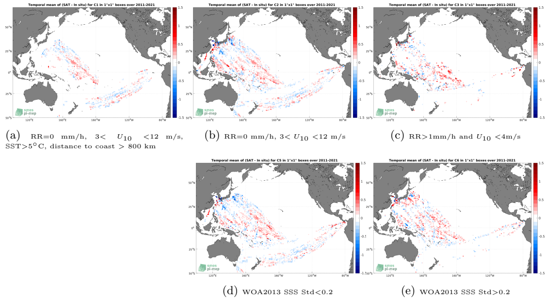
Figure 12: Temporal mean gridded over spatial boxes of size 1^\circ \times 1^\circ of \Delta\text{SSS} (SMOS SSS L4 v2 - Daily (BEC) - TSG (LEGOS-DM)) for 5 different subdatasets corresponding to:RR=0 mm/h, 3 < U_{10} < 12 m/s, SST >5^\circ\text{C} , distance to coast > 800 km (a), RR=0 mm/h, 3 < U_{10} < 12 m/s (b), RR >1 mm/h and U_{10} < 4 m/s (c), WOA2013 SSS Std <0.2 (d), WOA2013 SSS Std >0.2 (e).
