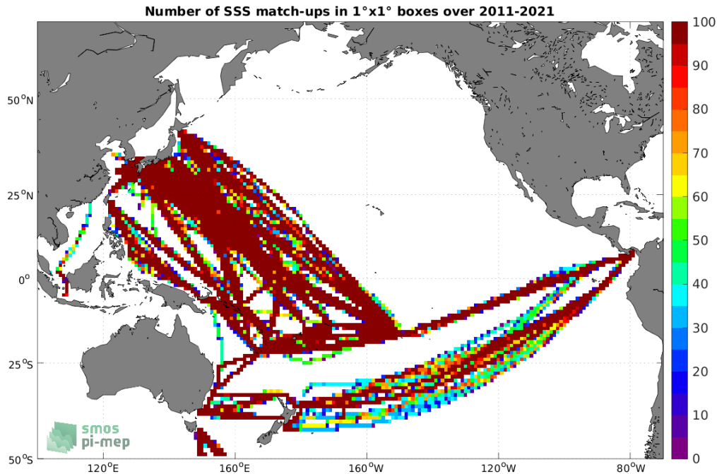
Figure 4: Number of SSS match-ups between TSG (LEGOS-DM) SSS and the SMOS SSS L4 v2 - Daily (BEC) SSS product for the Pacific Ocean Pi-MEP region over 1^\circ \times 1^\circ boxes and for the full satellite product period.
