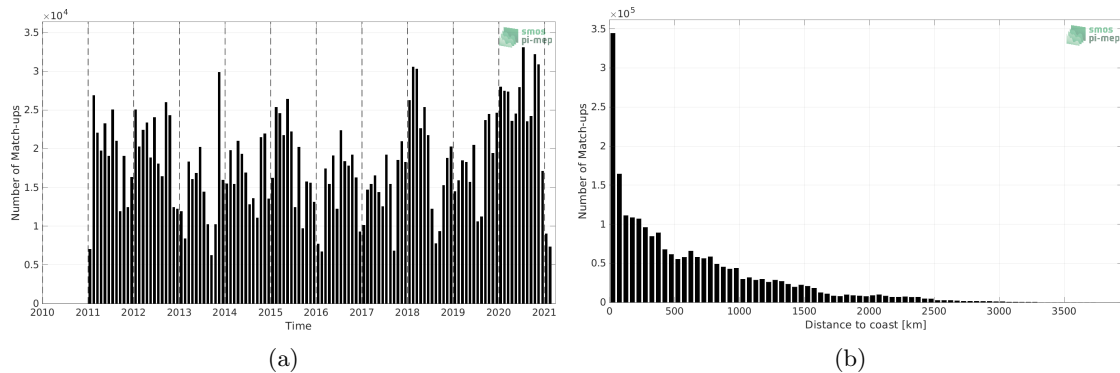
Figure 1: Number of match-ups between TSG (LEGOS-DM) and SMOS SSS L4 v2 - Daily (BEC) SSS as a function of time (a) and as function of the distance to coast (b) over the Pacific Ocean Pi-MEP region and for the full satellite product period.
