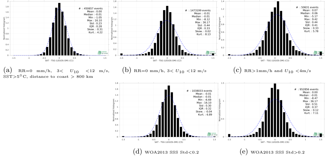
Figure 13: Normalized histogram of \Delta SSS (SMOS SSS L4 v2 - Daily (BEC) - TSG (LEGOS-DM)) for 5 different subdatasets corresponding to: RR=0 mm/h, 3 < U_{10} < 12 m/s, SST > 5°C, distance to coast > 800 km (a), RR=0 mm/h, 3 < U_{10} < 12 m/s (b), RR > 1mm/h and U_{10} < 4 m/s (c), WOA2013 SSS Std < 0.2 (d), WOA2013 SSS Std > 0.2 (e).
