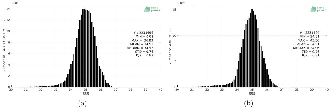
Figure 2: Histograms of SSS from TSG (LEGOS-DM) (a) and SMOS SSS L4 v2 - Daily (BEC) (b) considering all match-up pairs per bins of 0.1 over the Pacific Ocean Pi-MEP region and for the full satellite product period.
