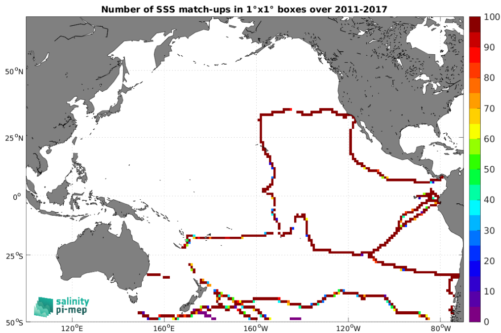
Figure 5: Number of SSS match-ups between TSG (GOSUD-Sailing-ship) SSS and the SMOS SSS L4 v2 - Daily (BEC) SSS product for the Pacific Ocean Pi-MEP region over 1^\circ \times 1^\circ boxes and for the full satellite product period.
