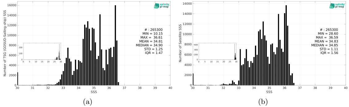
Figure 3: Histograms of SSS from TSG (GOSUD-Sailing-ship) (a) and SMOS SSS L4 v2 - Daily (BEC) (b) considering all match-up pairs per bins of 0.1 over the Pacific Ocean Pi-MEP region and for the full satellite product period.
