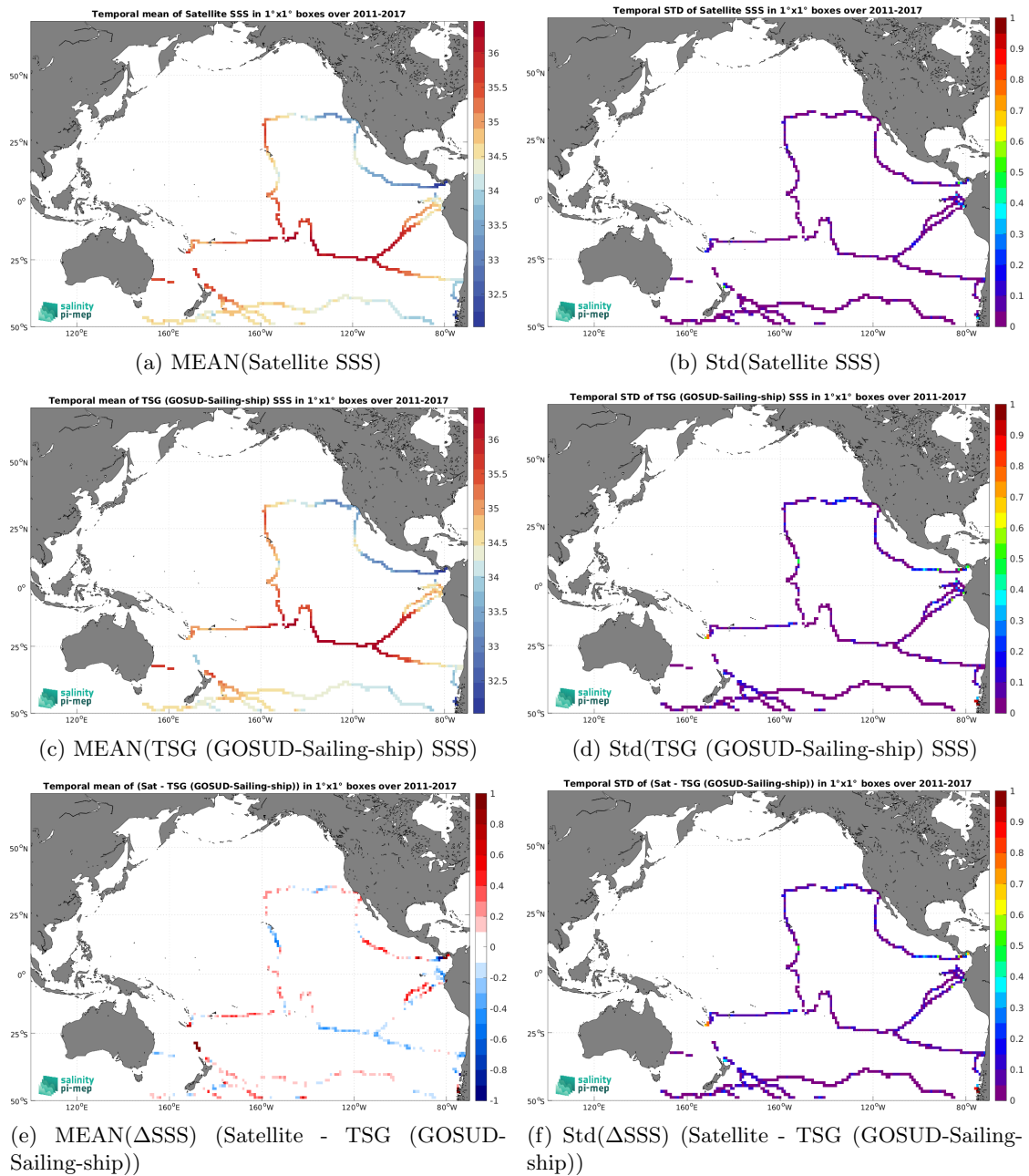
Figure 7: Temporal mean (left) and Std (right) of SSS from SMOS SSS L4 v2 - Daily (BEC) (top), TSG (GOSUD-Sailing-ship) (middle), and of \Delta SSS (Satellite - TSG (GOSUD-Sailing-ship)). Only match-up pairs are used to generate these maps.
