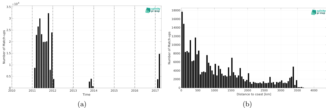
Figure 2: Number of match-ups between TSG (GOSUD-Sailing-ship) and SMOS SSS L4 v2 - Daily (BEC) SSS as a function of time (a) and as function of the distance to coast (b) over the Pacific Ocean Pi-MEP region and for the full satellite product period.
