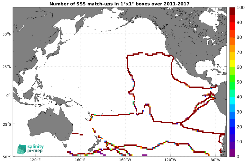
Figure 4: Number of SSS match-ups between TSG (GOSUD-Sailing-ship) SSS and the SMOS SSS L4 v2 - Daily (BEC) SSS product for the Pacific Ocean Pi-MEP region over 1°x1° boxes and for the full satellite product period.
