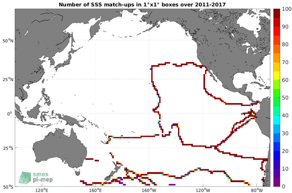
Figure 4: Number of SSS match-ups between TSG (GOSUD-Sailing-ship) SSS and the SMOS SSS L4 v2 - Daily (BEC) SSS product for the Pacific Ocean Pi-MEP region over 1^\circ \times 1^\circ boxes and for the full satellite product period.
