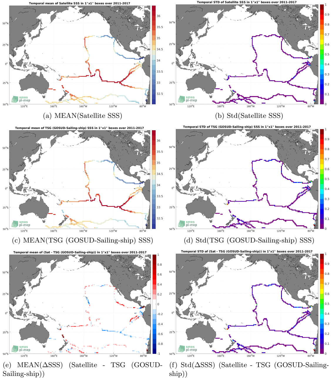
Figure 6: Temporal mean (left) and Std (right) of SSS from SMOS SSS L4 v2 - Daily (BEC) (top), TSG (GOSUD-Sailing-ship) (middle), and of \Delta SSS (Satellite - TSG (GOSUD-Sailing-ship)). Only match-up pairs are used to generate these maps.
