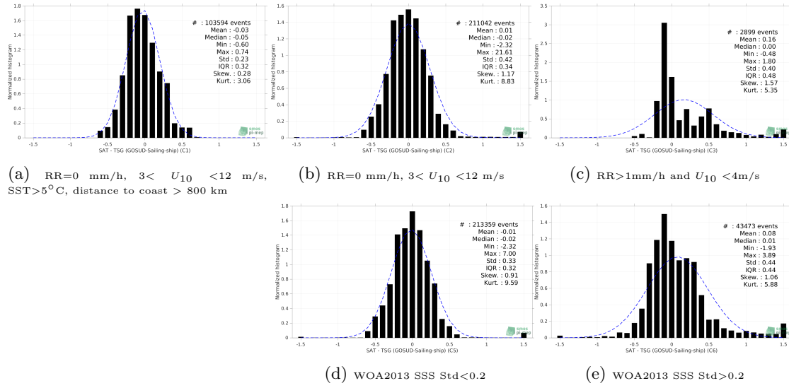
Figure 13: Normalized histogram of \Delta SSS (SMOS SSS L4 v2 - Daily (BEC) - TSG (GOSUD-Sailing-ship)) for 5 different subdatasets corresponding to: RR=0 mm/h, 3 < U_{10} < 12 m/s, SST >5^{\circ} C, distance to coast > 800 km (a), RR=0 mm/h, 3 < U_{10} < 12 m/s (b), RR >1 mm/h and U_{10} < 4 m/s (c), WOA2013 SSS Std <0.2 (d), WOA2013 SSS Std >0.2 (e).
