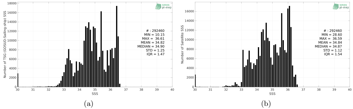
Figure 2: Histograms of SSS from TSG (GOSUD-Sailing-ship) (a) and SMOS SSS L4 v2 - Daily (BEC) (b) considering all match-up pairs per bins of 0.1 over the Pacific Ocean Pi-MEP region and for the full satellite product period.
