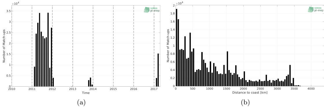
Figure 1: Number of match-ups between TSG (GOSUD-Sailing-ship) and SMOS SSS L4 v2 - Daily (BEC) SSS as a function of time (a) and as function of the distance to coast (b) over the Pacific Ocean Pi-MEP region and for the full satellite product period.
