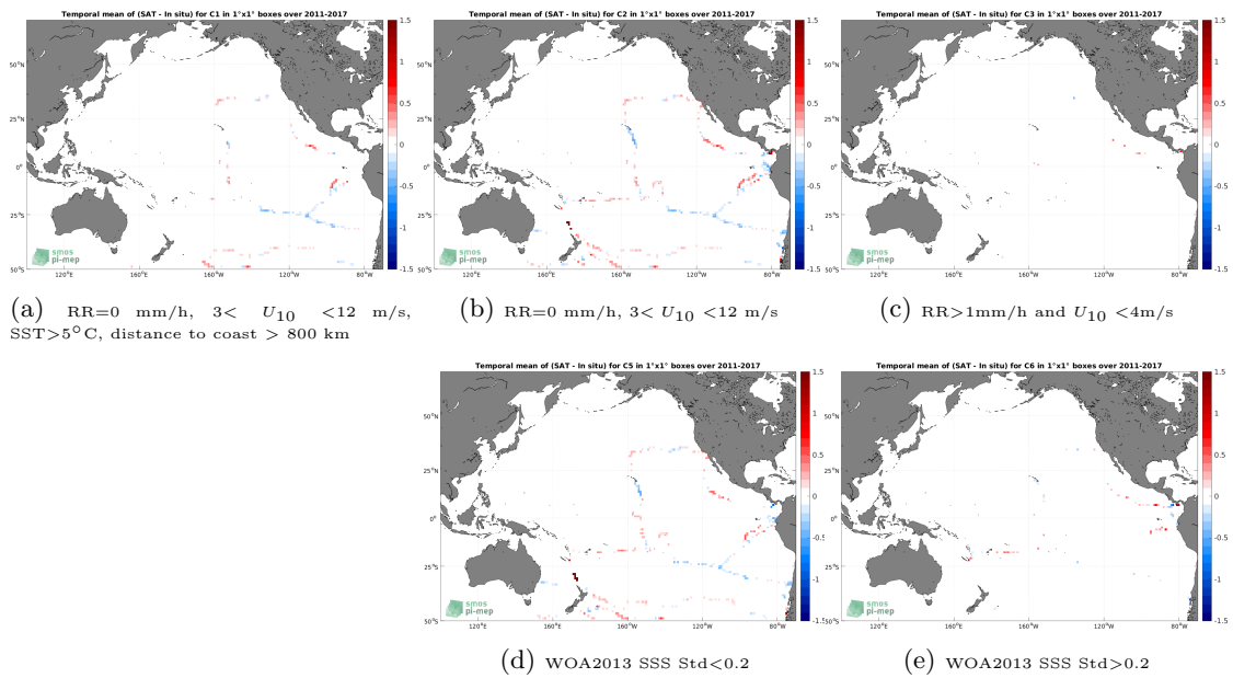
Figure 12: Temporal mean gridded over spatial boxes of size 1^\circ \times 1^\circ of \Delta SSS (SMOS SSS L4 v2 - Daily (BEC) - TSG (GOSUD-Sailing-ship)) for 5 different subdatasets corresponding to:RR=0 mm/h, 3 < U_{10} < 12 m/s, SST > 5^\circ C , distance to coast > 800 km (a), RR=0 mm/h, 3 < U_{10} < 12 m/s (b), RR>1mm/h and U_{10} < 4 m/s (c), WOA2013 SSS Std<0.2 (d), WOA2013 SSS Std>0.2 (e).
