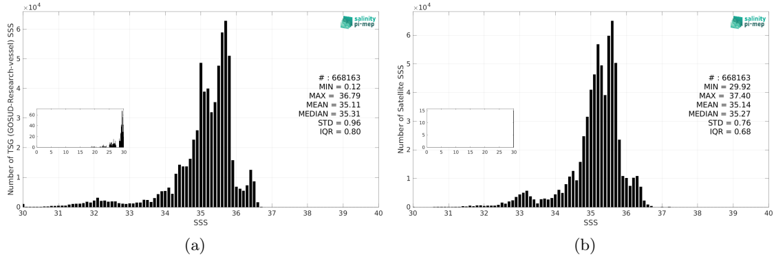
Figure 3: Histograms of SSS from TSG (GOSUD-Research-vessel) (a) and SMOS SSS L4 v2 - Daily (BEC) (b) considering all match-up pairs per bins of 0.1 over the Pacific Ocean Pi-MEP region and for the full satellite product period.
