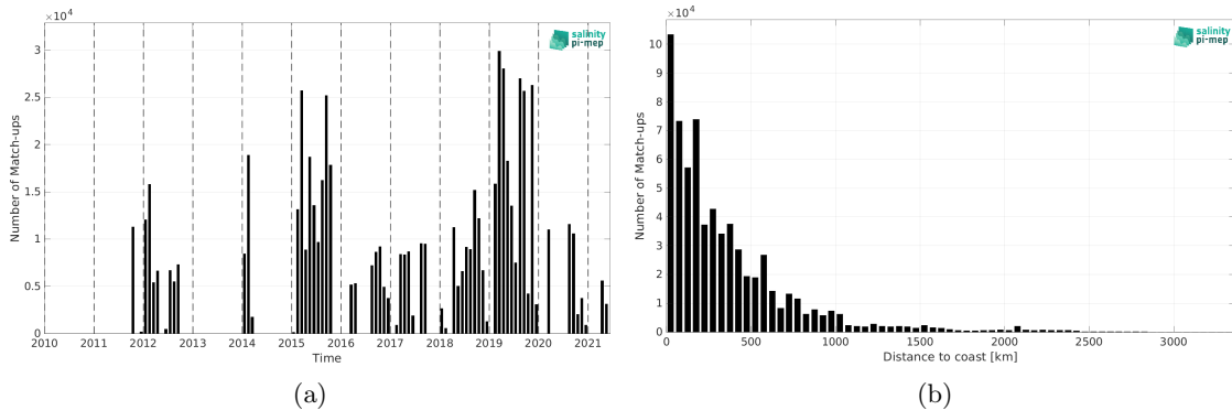
Figure 2: Number of match-ups between TSG (GOSUD-Research-vessel) and SMOS SSS L4 v2 - Daily (BEC) SSS as a function of time (a) and as function of the distance to coast (b) over the Pacific Ocean Pi-MEP region and for the full satellite product period.
