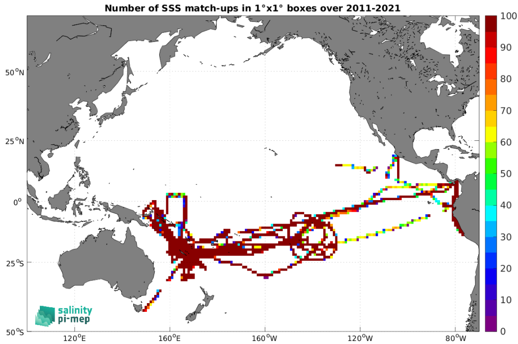
Figure 5: Number of SSS match-ups between TSG (GOSUD-Research-vessel) SSS and the SMOS SSS L4 v2 - Daily (BEC) SSS product for the Pacific Ocean Pi-MEP region over 1^\circ \times 1^\circ boxes and for the full satellite product period.
