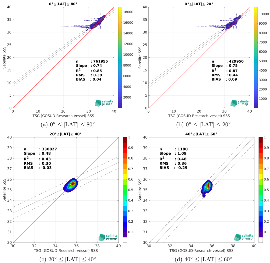
Figure 9: Contour maps of the concentration of SMOS SSS L4 v2 - Daily (BEC) SSS (y-axis) versus TSG (GOSUD-Research-vessel) SSS (x-axis) at match-up pairs for different latitude bands. For each plot, the red line shows x=y . The black thin and dashed lines indicate a linear fit through the data cloud and the \pm 95\% confidence levels, respectively. The number match-up pairs n , the slope and R^2 coefficient of the linear fit, the root mean square (RMS) and the mean bias between satellite and in situ data are indicated for each latitude band in each plots.
