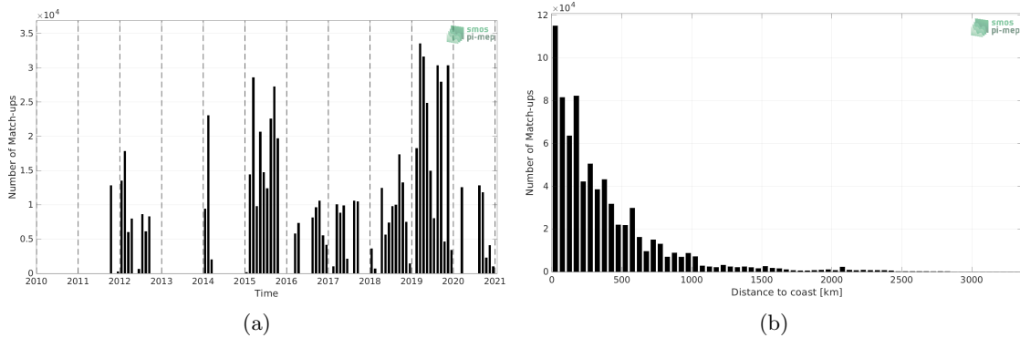
Figure 1: Number of match-ups between TSG (GOSUD-Research-vessel) and SMOS SSS L4 v2 - Daily (BEC) SSS as a function of time (a) and as function of the distance to coast (b) over the Pacific Ocean Pi-MEP region and for the full satellite product period.
