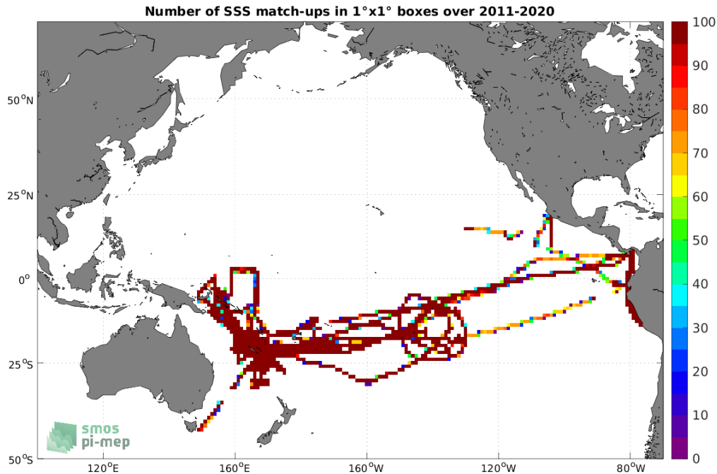
Figure 4: Number of SSS match-ups between TSG (GOSUD-Research-vessel) SSS and the SMOS SSS L4 v2 - Daily (BEC) SSS product for the Pacific Ocean Pi-MEP region over 1^\circ \times 1^\circ boxes and for the full satellite product period.
