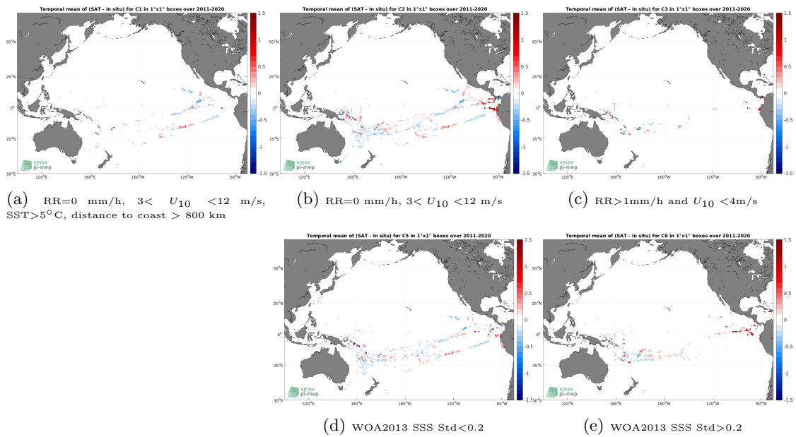
Figure 12: Temporal mean gridded over spatial boxes of size 1^\circ \times 1^\circ of \Delta SSS (SMOS SSS L4 v2 - Daily (BEC) - TSG (GOSUD-Research-vessel)) for 5 different subdatasets corresponding to:RR=0 mm/h, 3 < U_{10} < 12 m/s, SST>5°C, distance to coast > 800 km (a), RR=0 mm/h, 3 < U_{10} < 12 m/s (b), RR>1mm/h and U_{10} < 4 m/s (c), WOA2013 SSS Std<0.2 (d), WOA2013 SSS Std>0.2 (e).
