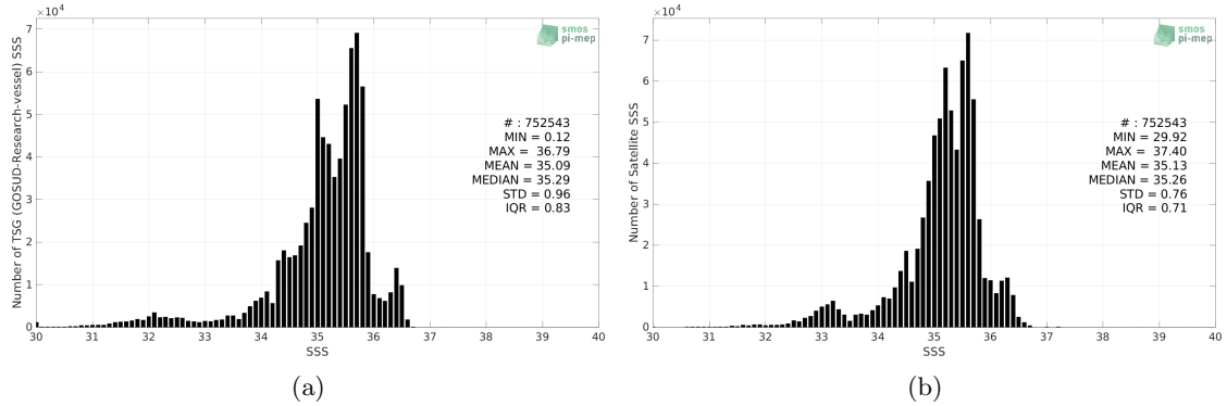
Figure 2: Histograms of SSS from TSG (GOSUD-Research-vessel) (a) and SMOS SSS L4 v2 - Daily (BEC) (b) considering all match-up pairs per bins of 0.1 over the Pacific Ocean Pi-MEP region and for the full satellite product period.
